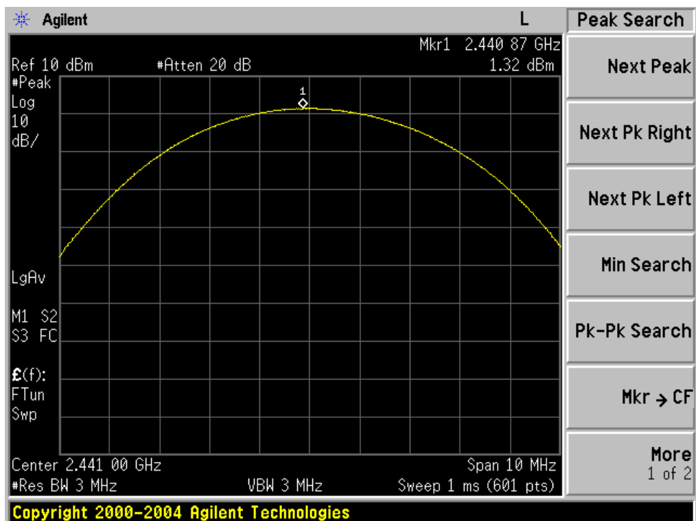
Peak output Power plot on channel 39
