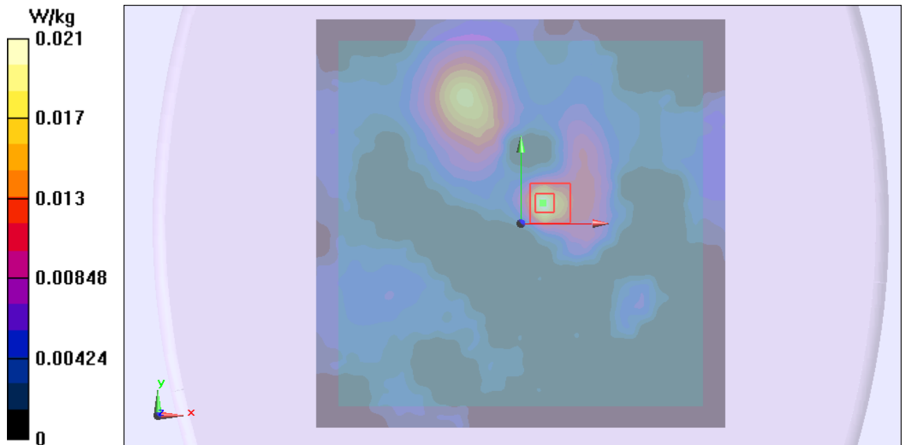
Figure 7 802.11b Test Position 1 Channel 11
