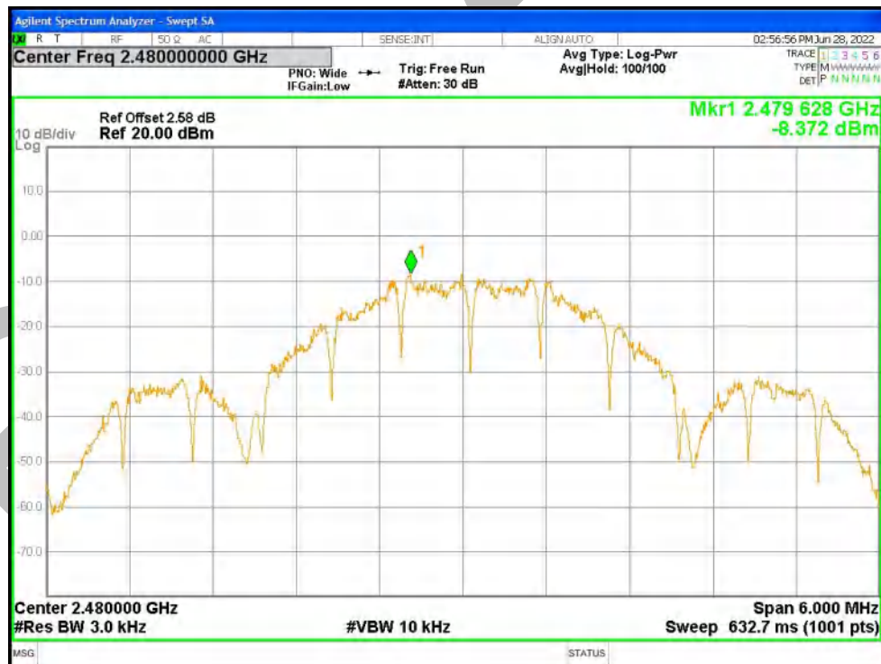
PSD NVNT THREAD 2480MHz Ant1
