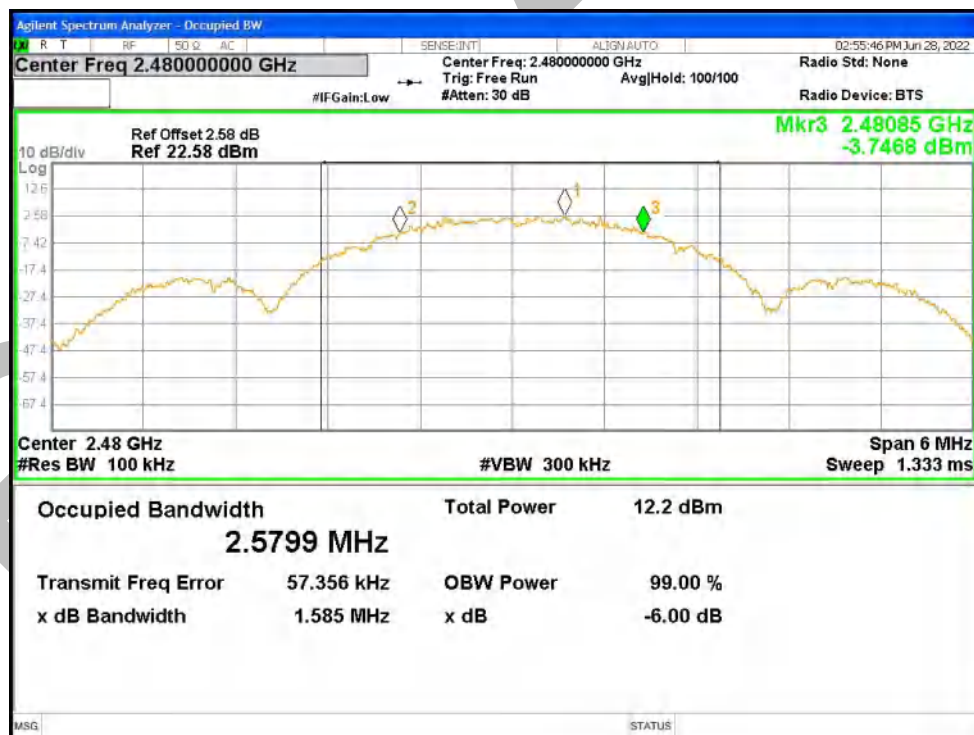
-6dB Bandwidth NVNT THREAD 2480MHz Ant1
