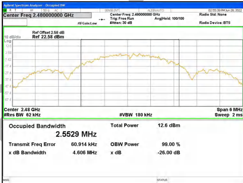
OBW NVNT THREAD 2480MHz Ant1
