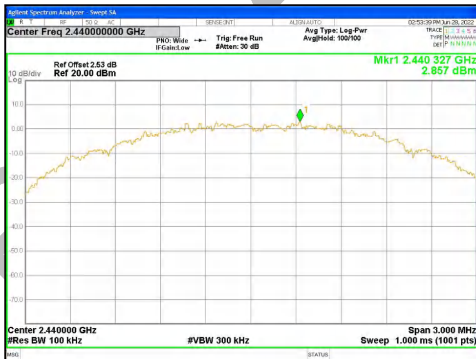
Tx. Spurious NVNT THREAD 2440MHz Ant1 Emission
