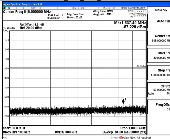
DH5_Ant1_2402_30~1000
