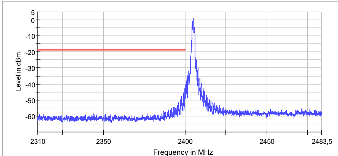
Screenshot: Lower band edge sweep
