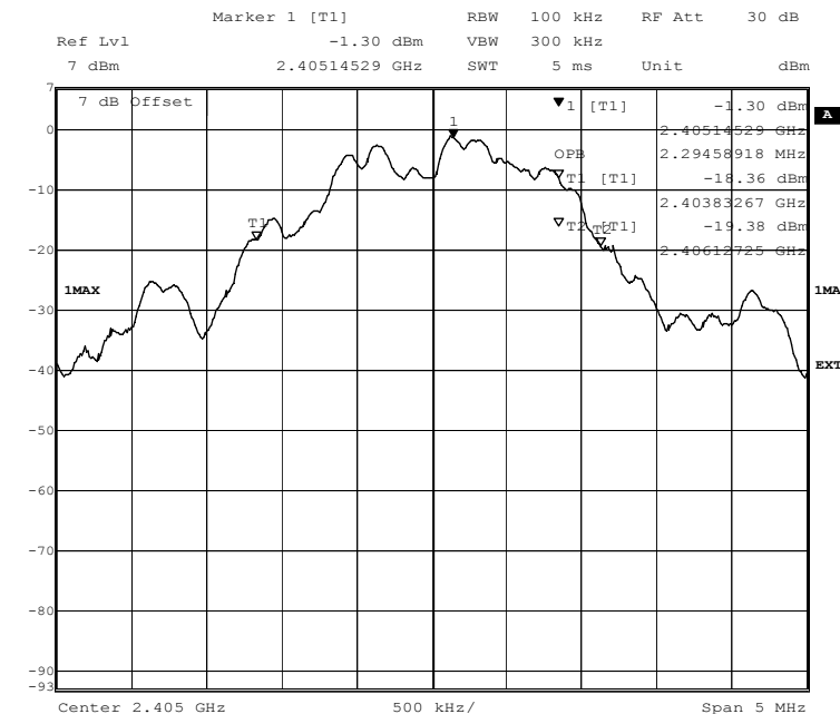
Screenshot: 99 % bandwidth Measurement
