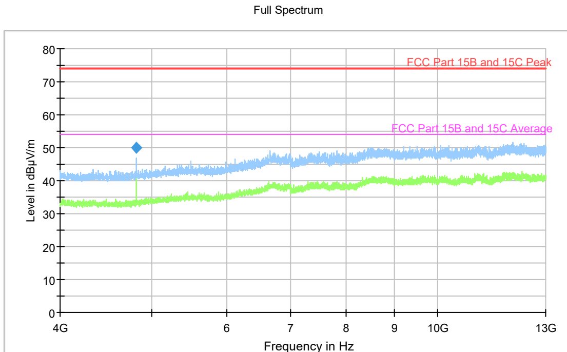
Diagram, Peak overview sweep, 4– 13 GHz at 3 m distance. TX. Emissions below 4000 MHz are attenuated by high-pass filter K&L 4410-X4500/18000-0.
