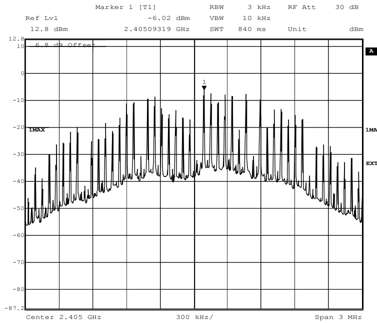
Screenshot: Peak power spectral density
