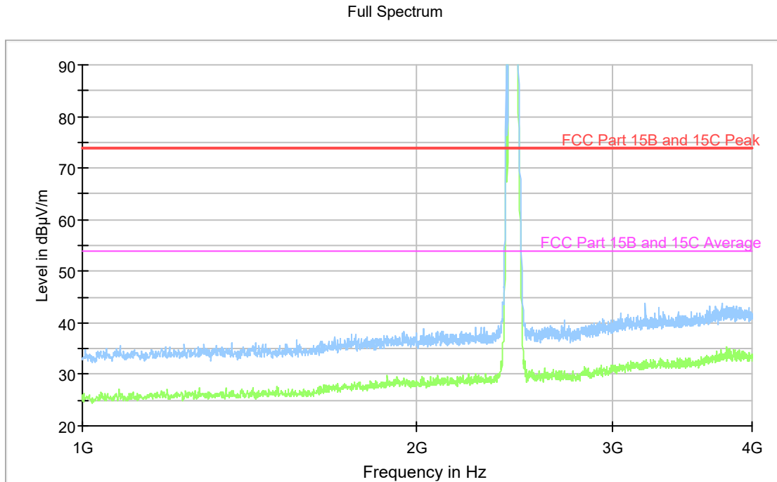
Diagram, Peak overview sweep, 1– 4 GHz at 3 m distance. TX. Carrier is attenuated by band rejection filter K&L 6N45-2450/T 100-0/0.
