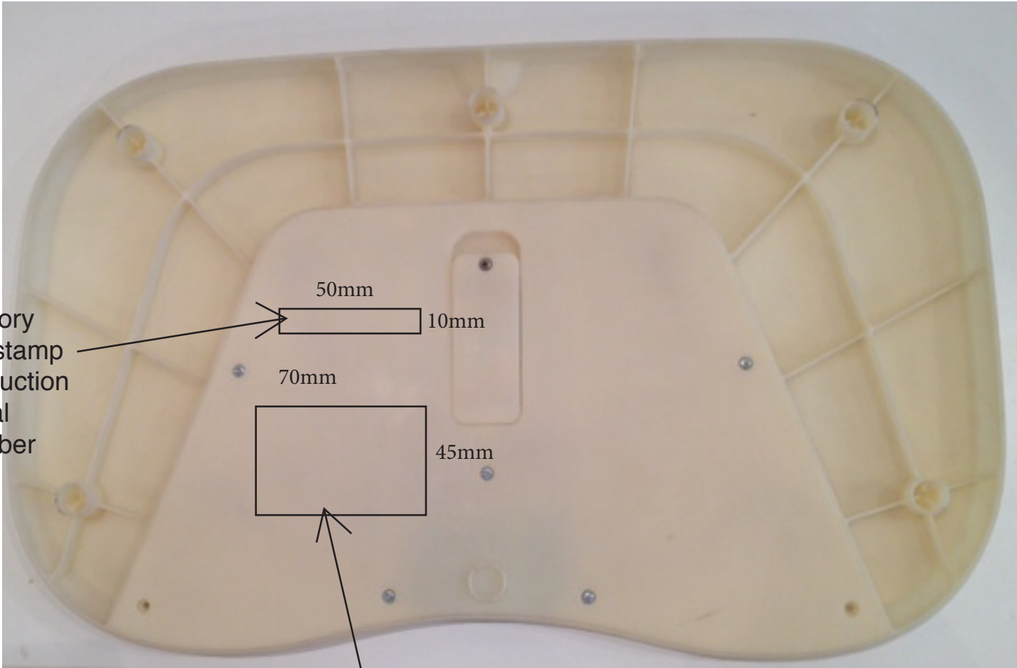
Label engraved in a mould insert (already prepared)
