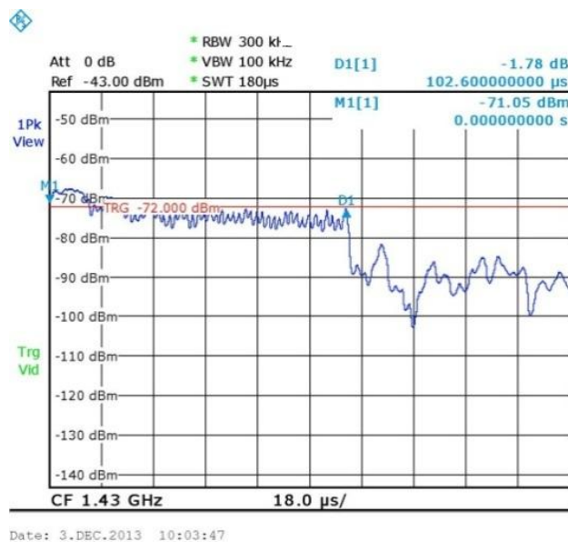
Figure 66 — Dwell time [5X100usec=500usec/sec]
