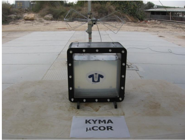
Radiated Emission Test as Stand-alone
