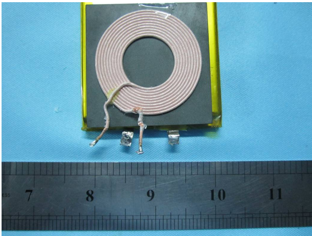
Coil Antenna - Top View
