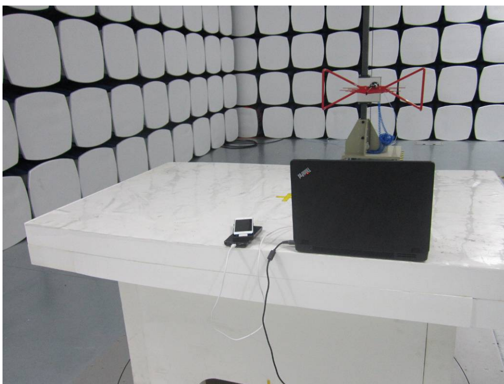
Radiated Spurious Emissions Test Setup Above 30 MHz - Front View
