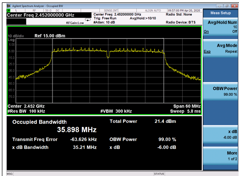
(Channel 9, 802.11n(HT40))
