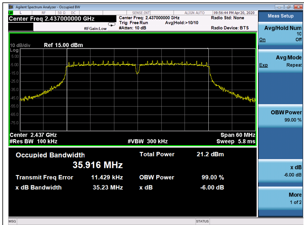
(Channel 6, 802.11n(HT40))
