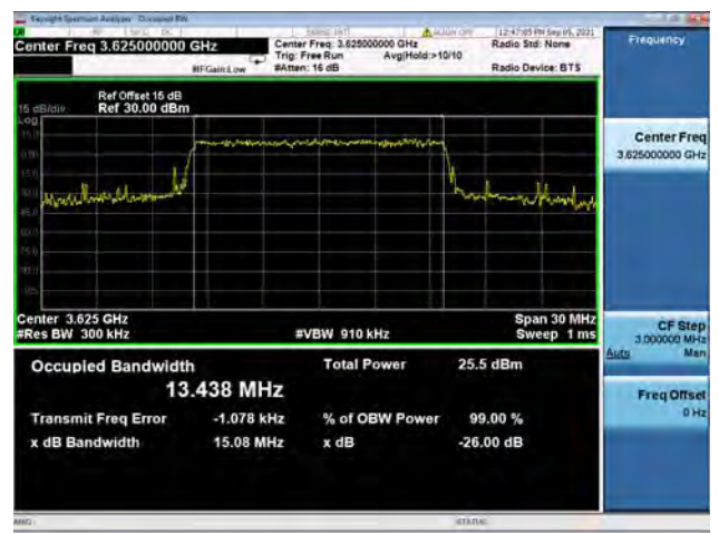
Band48 / 15MHz / Mid CH / 64QAM
