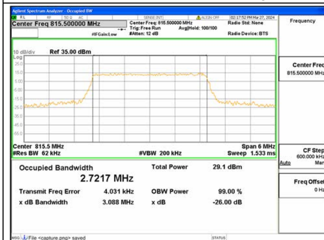
B26 Part90 / 3MHz / 16QAM/ Low CH
