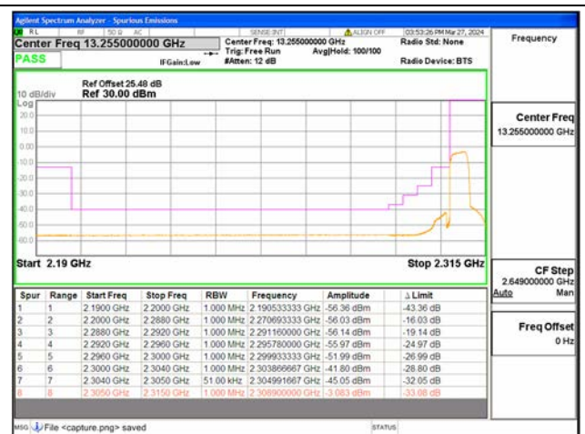
B30 / 5MHz / Low CH / QPSK / FULL RB
