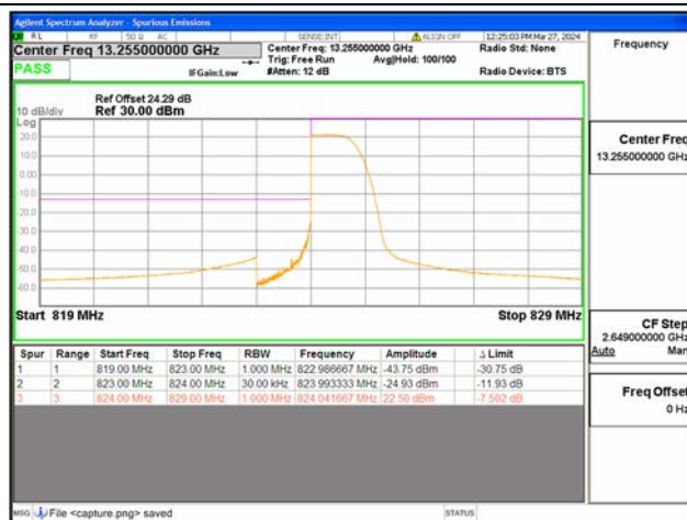
B26 Part22 / 3MHz / Low CH / QPSK / 1 RB
