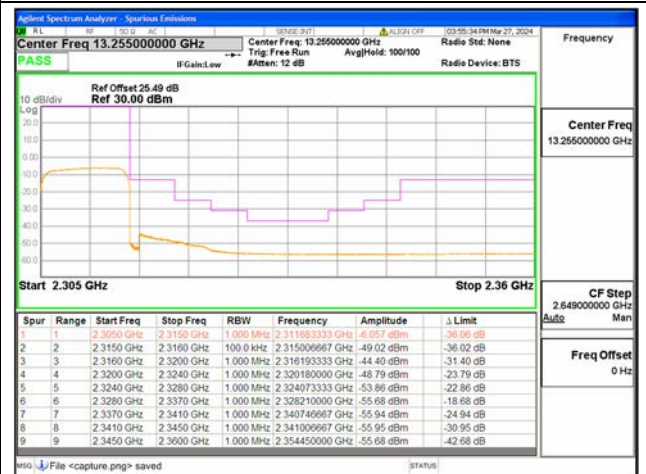
B30 / 10MHz / High CH / QPSK / FULL RB
