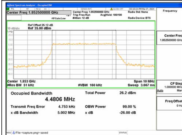
B25 / 5MHz / 64QAM/ Low CH
