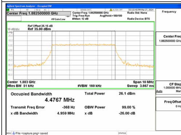
B25 / 5MHz / 16QAM/ Mid CH
