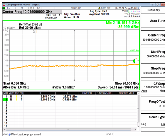
n77(3700-3980MHz) (30MHz-20GHz) 30M DFT-s-OFDM BPSK Inner 1RB Right Mid
