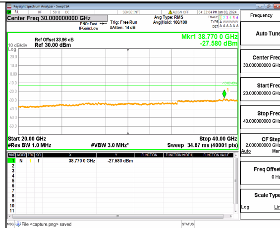
n77(3700-3980MHz) (20GHz-40GHz) 30M DFT-s-OFDM BPSK Inner 1RB Left Mid
