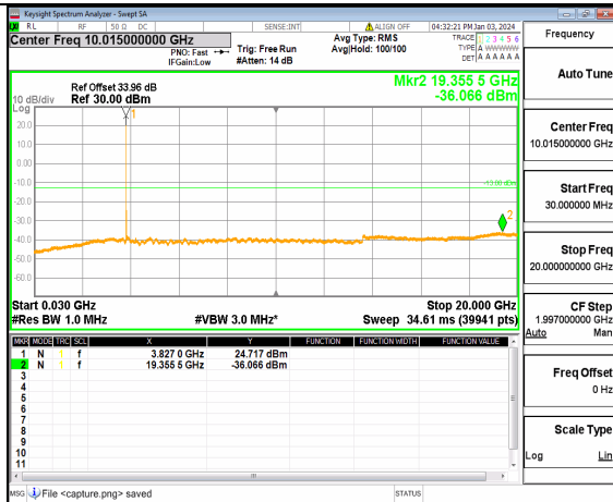
n77(3700-3980MHz) (30MHz-20GHz) 30M DFT-s-OFDM BPSK Inner 1RB Left Mid
