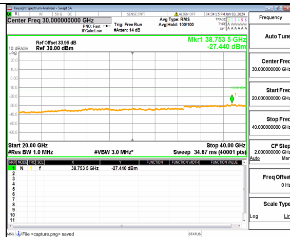
n77(3700-3980MHz) (20GHz-40GHz) 30M DFT-s-OFDM BPSK Inner 1RB Right Mid
