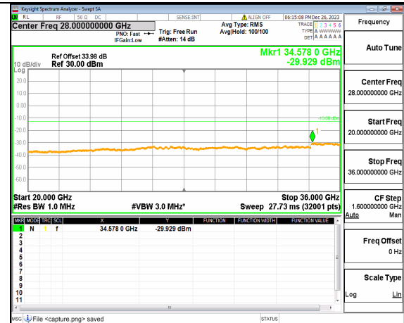
n77(3450-3550MHz) (20GHz-36GHz) 80M DFT-s-OFDM QPSK Inner_1RB_Right Mid
