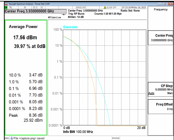
n77(3700-3980MHz) 100M DFT-s-OFDM 256QAM Outer_Full High
