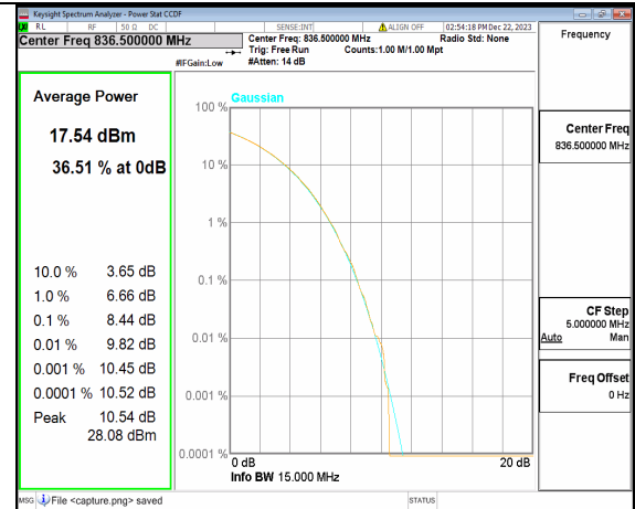
n5 15M CP-OFDM 256QAM Outer_Full Mid
