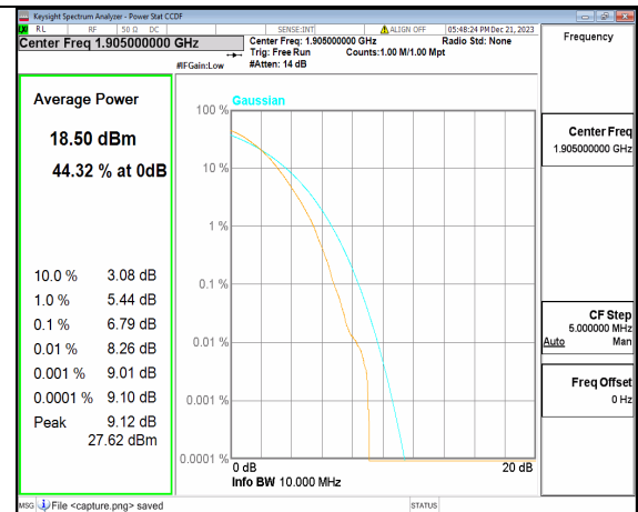
n2 10M DFT-s-OFDM 256QAM Outer_Full High
