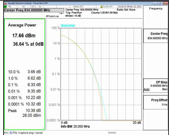
n5 20M CP-OFDM 256QAM Outer_Full Low
