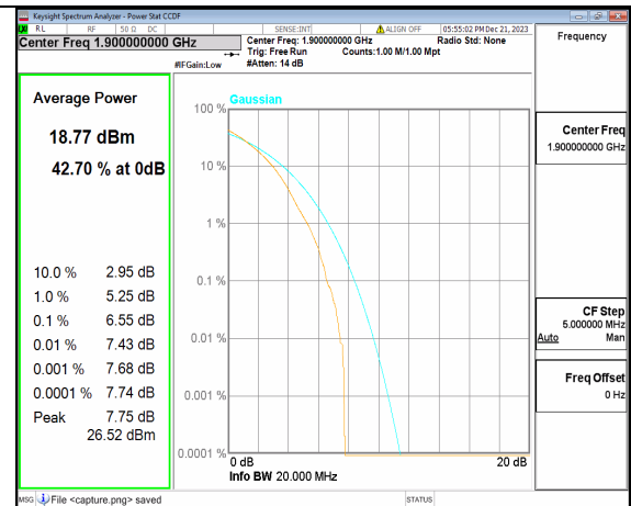
n2 20M DFT-s-OFDM 256QAM Outer_Full High
