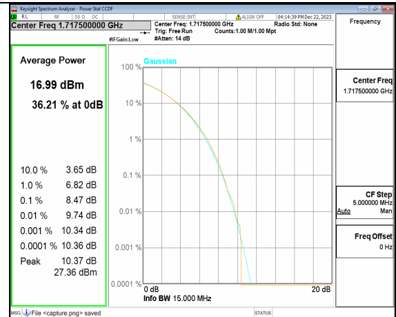
n66 15M CP-OFDM 256QAM Outer_Full Low
