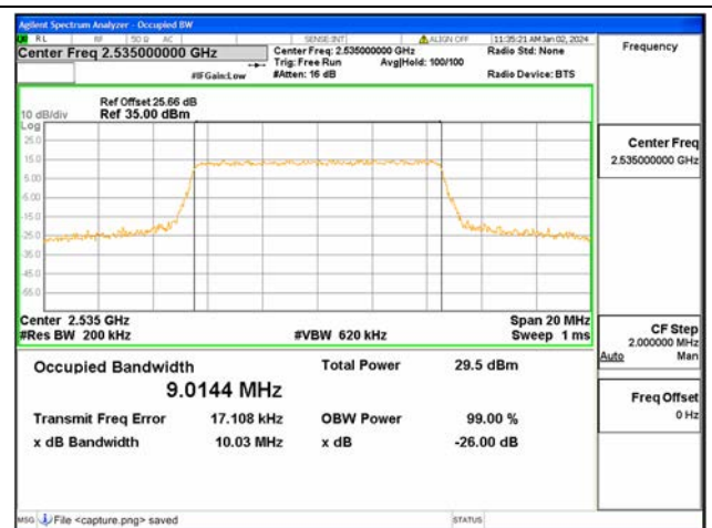
B7 / 10MHz / 16QAM/ Mid CH
