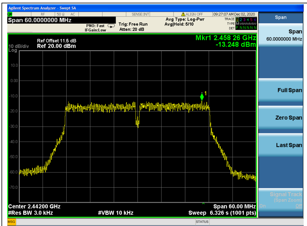
(Channel 7, 802.11n (HT40), ANT0)
