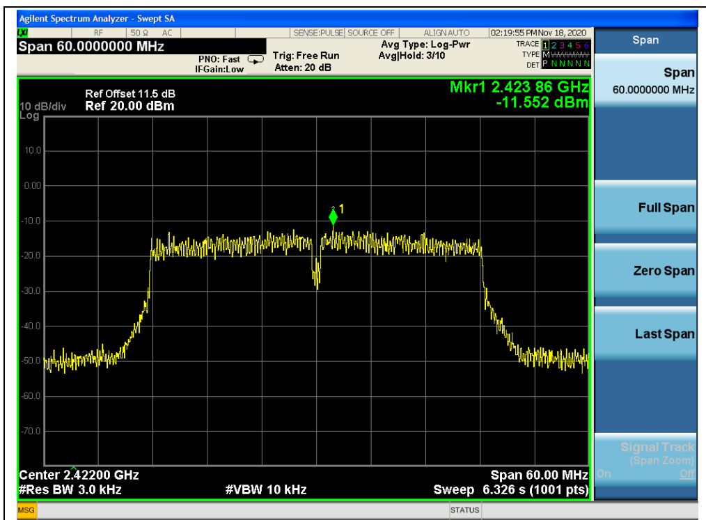
(Channel 3, 802.11n (HT40), ANT1)
