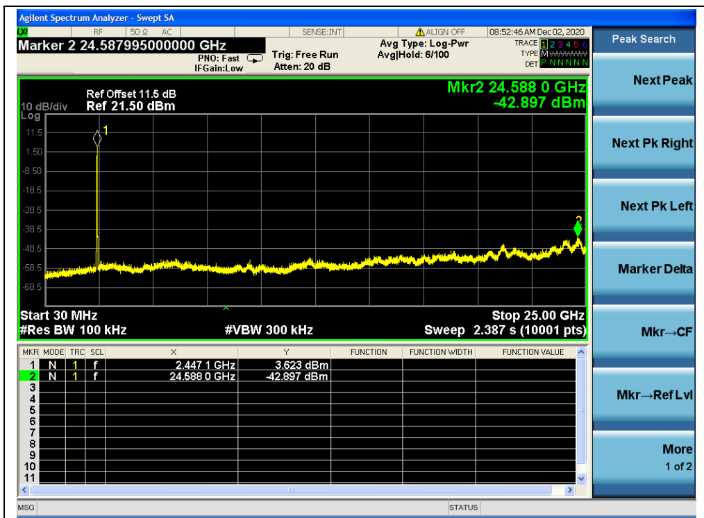
(30MHz to 25GHz, Channel 7, 802.11n (HT20))
