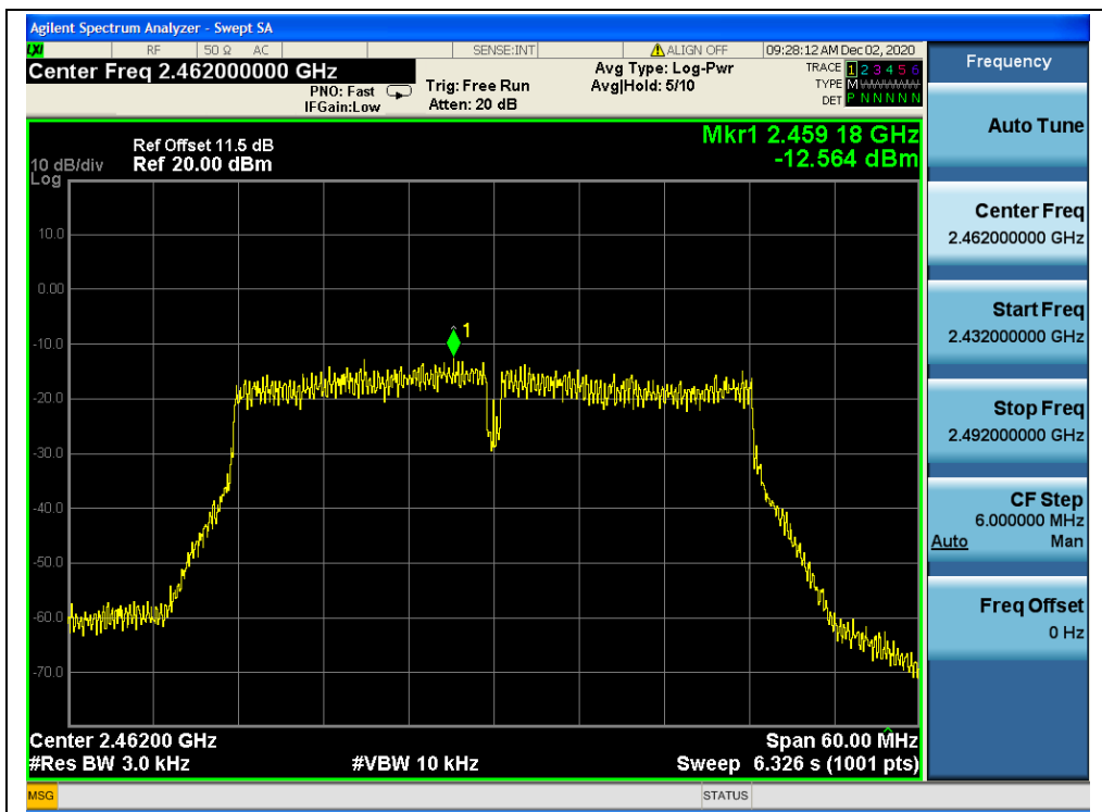
(Channel 11, 802.11n (HT40), ANT0)
