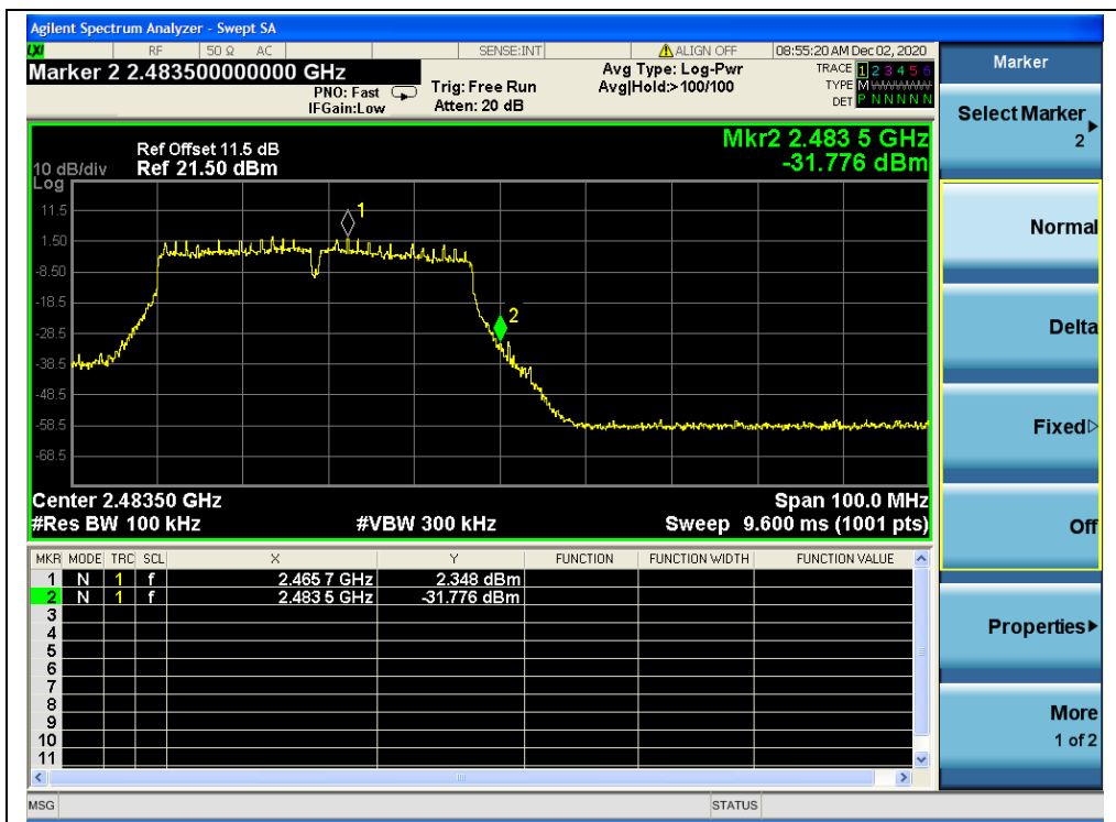
(Band Edge, Channel 11, 802.11n (HT40))
