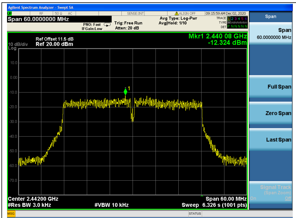
(Channel 7, 802.11n (HT40), ANT1)
