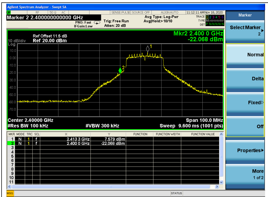
(Band Edge, Channel 1, 802.11n (HT20))
