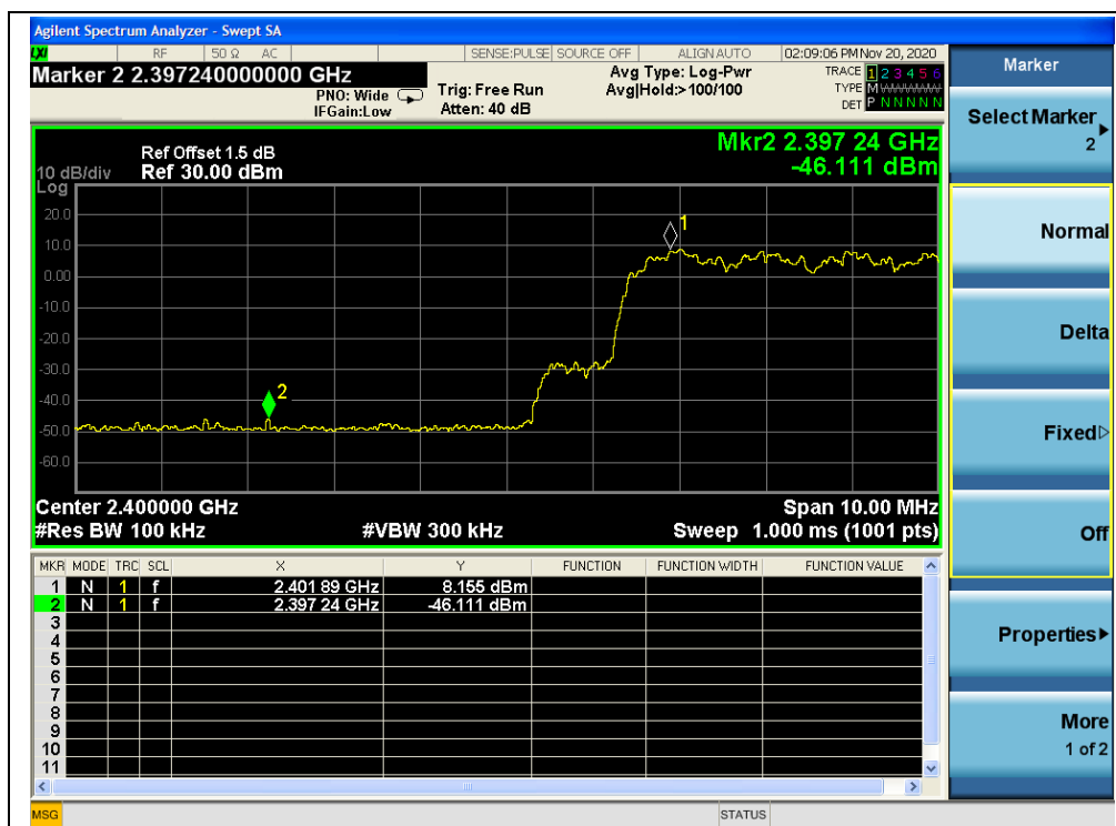
(Band edge with hopping on, Channel 0, 8-DPSK)
