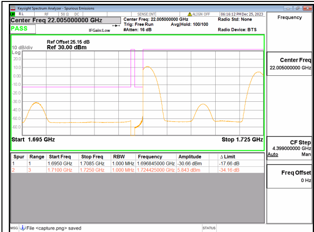
66B / 10+5MHz / Low CH / QPSK / 1#0-1#24
