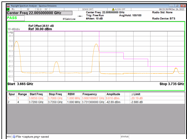
48C / 20+15MHz / High CH / QPSK / 1#0-1#74
