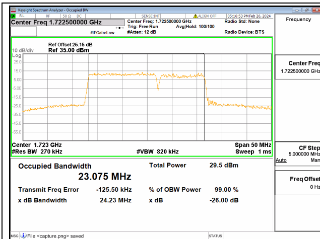
66C / 15+10MHz / 16QAM/ Low CH
