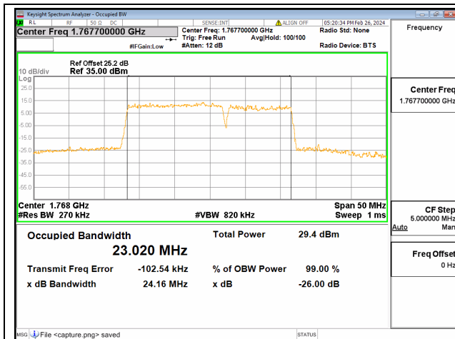
66C / 15+10MHz / 16QAM/ High CH
