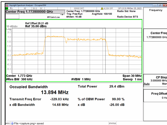
66B / 5+10MHz / 16QAM/ High CH
