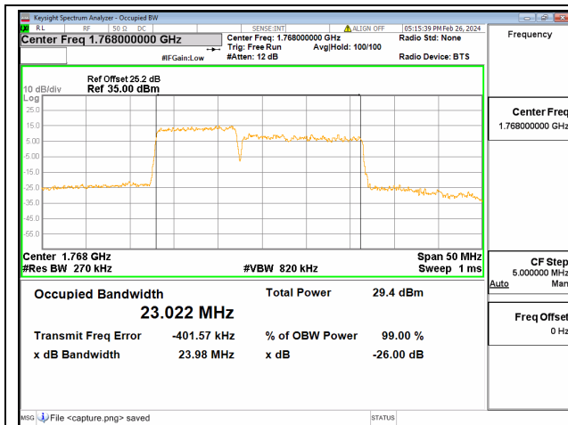
66C / 10+15MHz / 16QAM/ High CH
