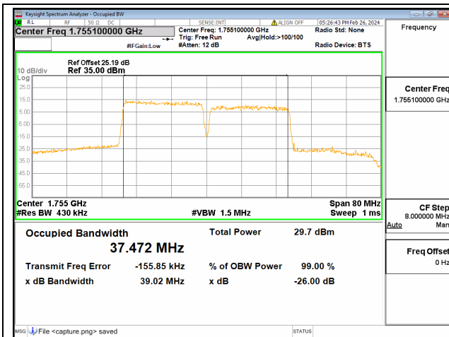
66C / 20+20MHz / 16QAM/ Mid CH
