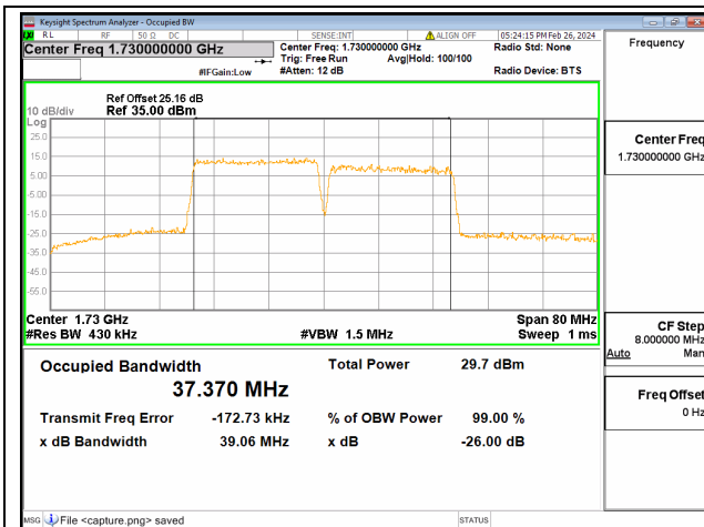
66C / 20+20MHz / 16QAM/ Low CH
