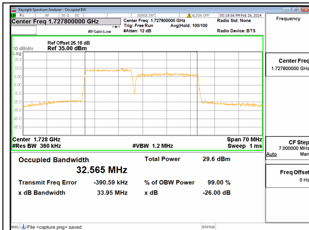
66C / 15+20MHz / 16QAM/ Low CH
