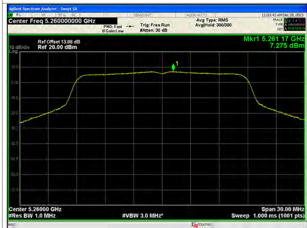
PSD NVNT ac20 5260MHz Ant2 SISO
