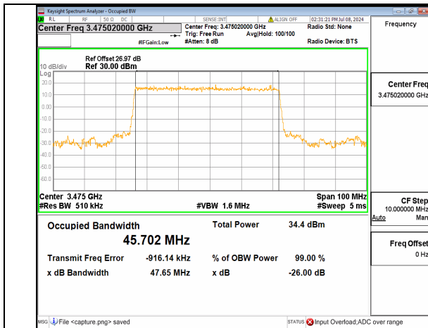
n77(3450-3550MHz) 50M DFT-s-OFDM BPSK Outer_Full Low
