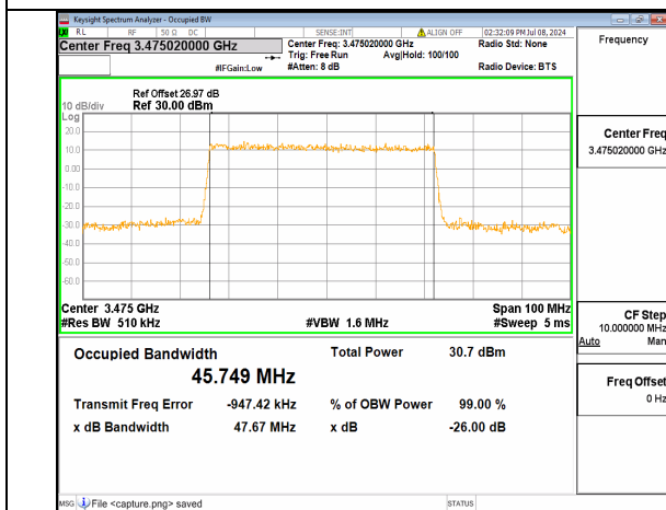
n77(3450-3550MHz) 50M DFT-s-OFDM 256QAM Outer_Full Low
