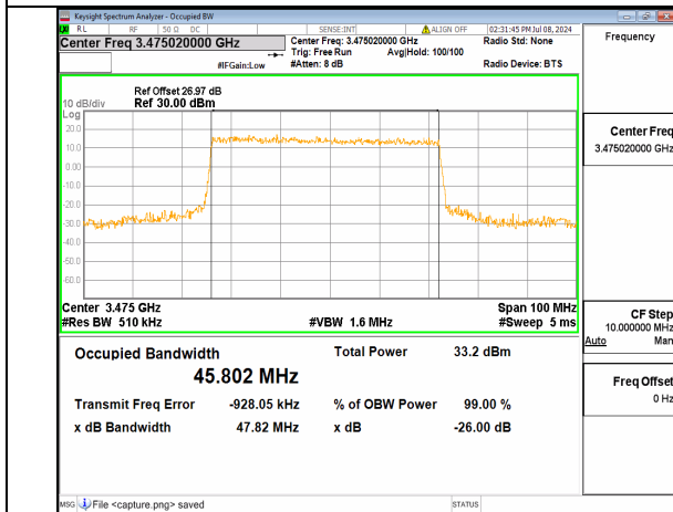
n77(3450-3550MHz) 50M DFT-s-OFDM 16QAM Outer_Full Low
