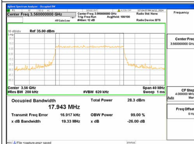
B48 / 20MHz / 16QAM/ Low CH
