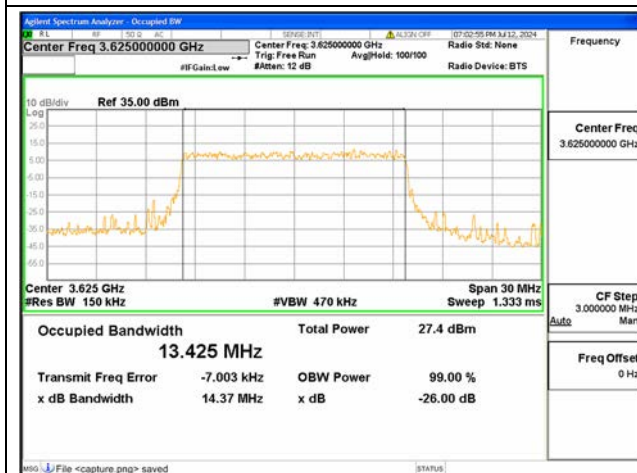
B48 / 15MHz / 16QAM/ Mid CH
