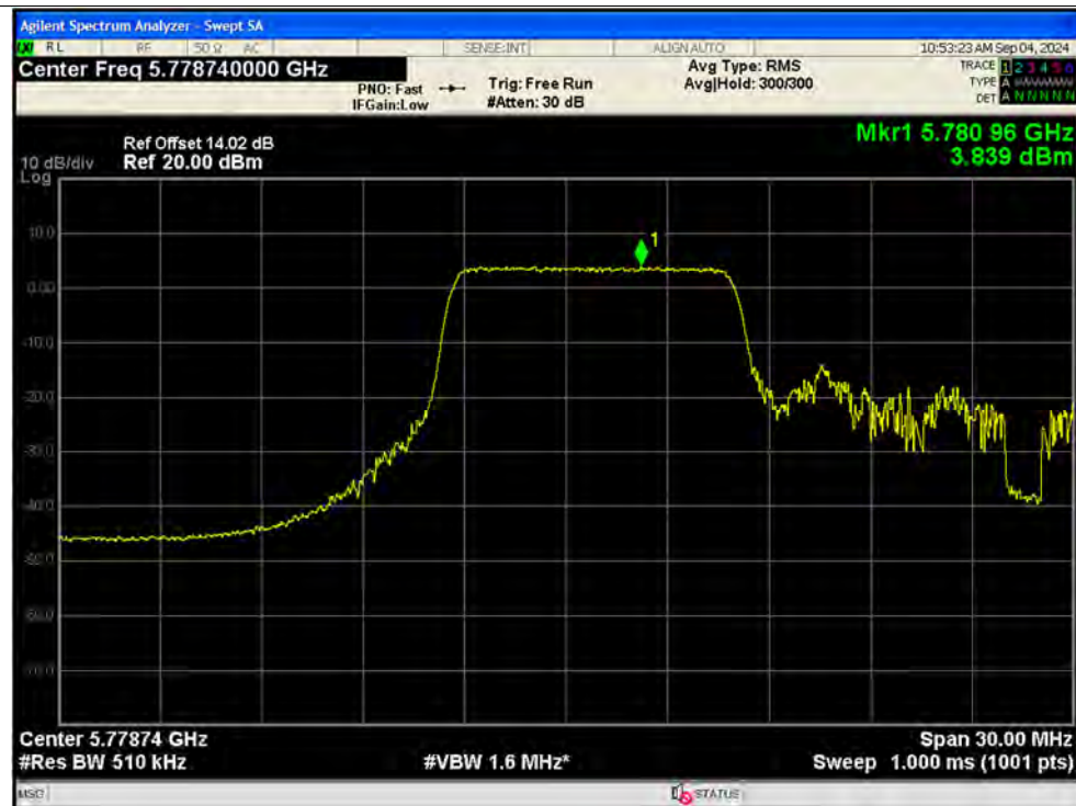
PSD NVNT ax20 106@53 5785MHz Ant2 MIMO
