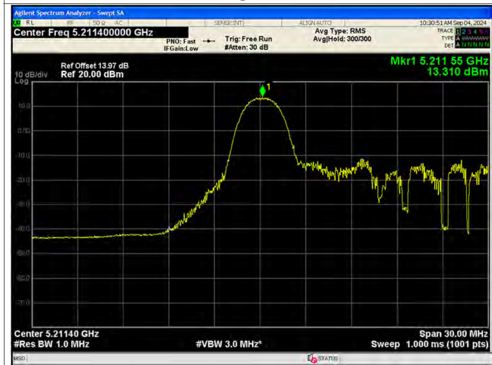
PSD NVNT ax20 26@0 5220MHz Ant2 MIMO
