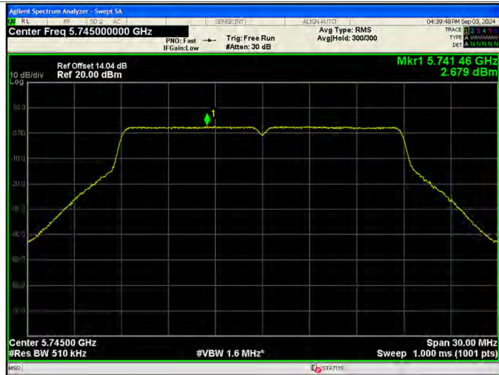
PSD NVNT n20 5745MHz Ant2 MIMO
