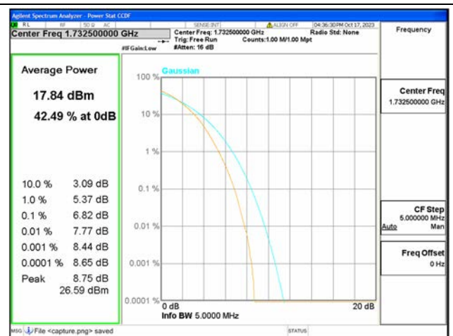
B4 / 5MHz / Mid CH / 256QAM
