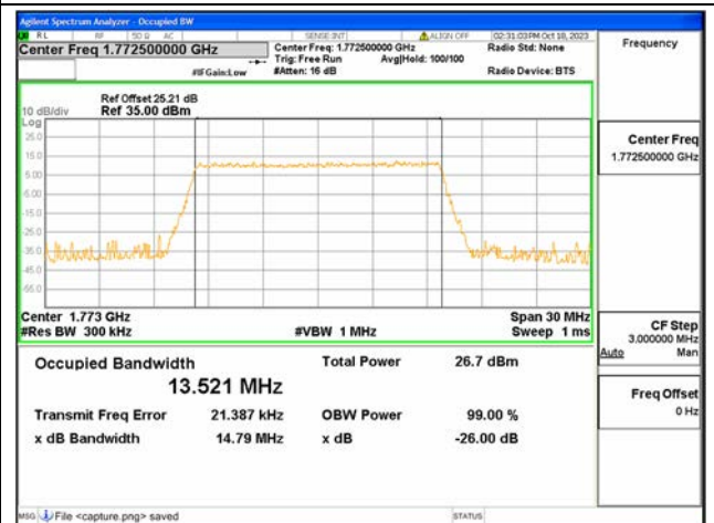
B66 / 15MHz / 256QAM/ High CH
