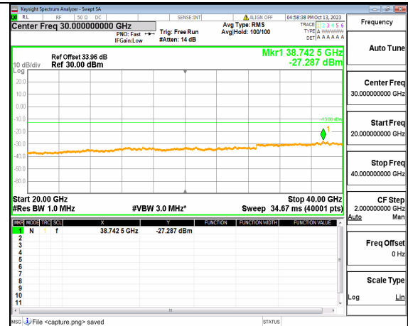
5A_n77(3700-3980MHz) (20GHz-40GHz) 60M DFT-s-OFDM QPSK Edge_1RB_Left Mid
