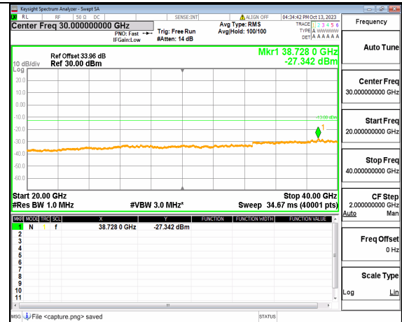
5A_n77(3700-3980MHz) (20GHz-40GHz) 50M DFT-s-OFDM QPSK Edge_1RB_Left Mid
