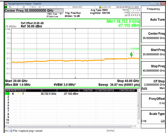
5A_n77(3700-3980MHz) (20GHz-40GHz) 50M DFT-s-OFDM QPSK Edge_1RB_Left High
