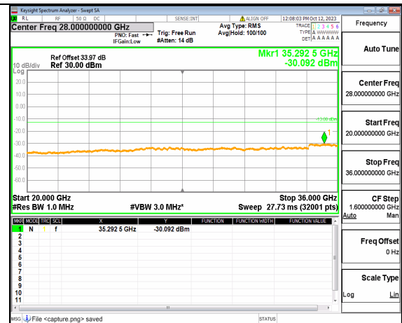
5A_n77(3450-3550MHz) (20GHz-36GHz) 70M DFT-s-OFDM BPSK Edge_1RB_Left Low
