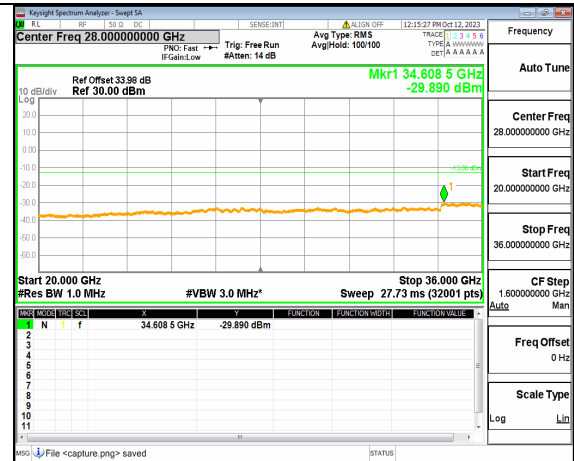
5A_n77(3450-3550MHz) (20GHz-36GHz) 70M DFT-s-OFDM BPSK Edge_1RB_Left Mid
