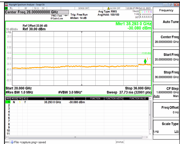
5A_n77(3450-3550MHz) (20GHz-36GHz) 70M DFT-s-OFDM QPSK Edge_1RB_Left High
