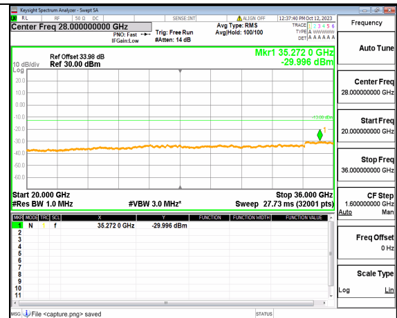
5A_n77(3450-3550MHz) (20GHz-36GHz) 80M DFT-s-OFDM BPSK Edge_1RB_Left Mid
