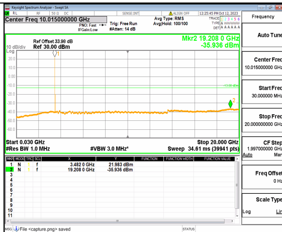
5A_n77(3450-3550MHz) (30MHz-20GHz) 70M DFT-s-OFDM QPSK Edge_1RB Left High
