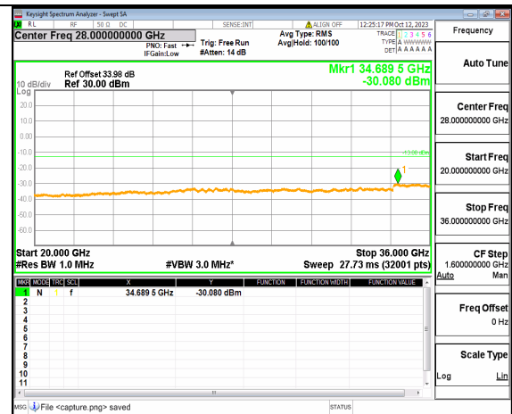
5A_n77(3450-3550MHz) (20GHz-36GHz) 70M DFT-s-OFDM QPSK Outer_Full High
