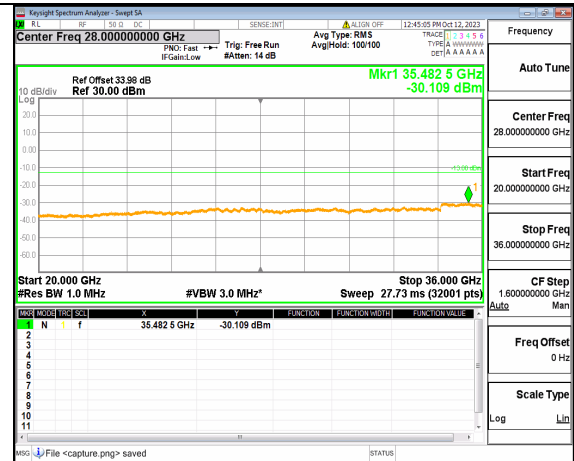
5A_n77(3450-3550MHz) (20GHz-36GHz) 80M DFT-s-OFDM BPSK Edge_1RB_Left High
