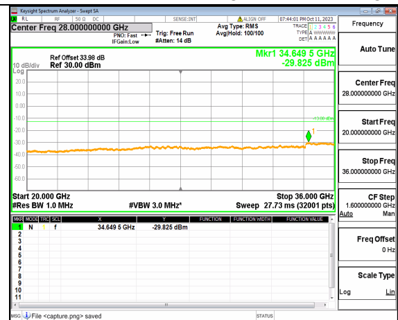
5A_n77(3450-3550MHz) (20GHz-36GHz) 30M DFT-s-OFDM QPSK Edge_1RB_Right High
