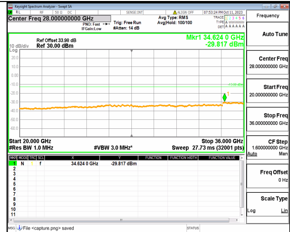
5A_n77(3450-3550MHz) (20GHz-36GHz) 40M DFT-s-OFDM BPSK Outer_Full Mid
