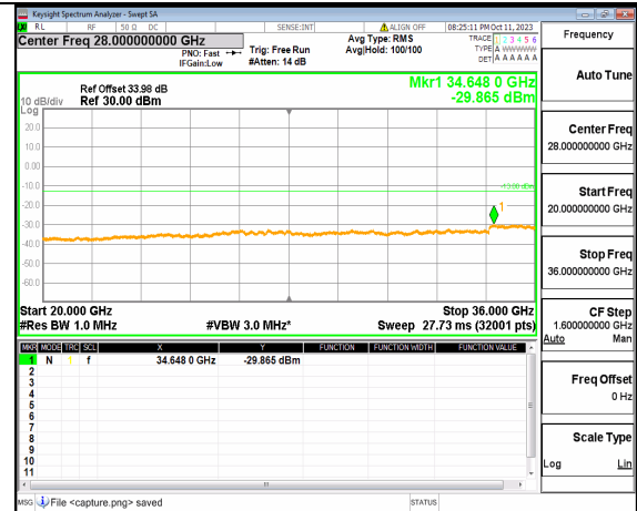
5A_n77(3450-3550MHz) (20GHz-36GHz) 50M DFT-s-OFDM BPSK Outer_Full High
