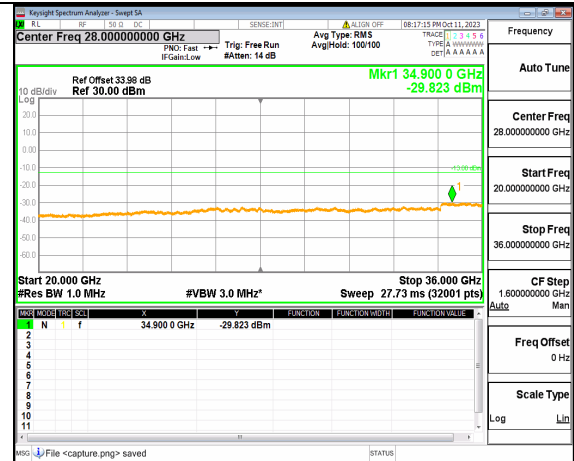
5A_n77(3450-3550MHz) (20GHz-36GHz) 50M DFT-s-OFDM BPSK Outer_Full Mid
