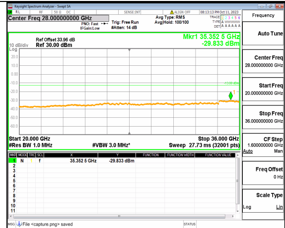
5A_n77(3450-3550MHz) (20GHz-36GHz) 50M DFT-s-OFDM QPSK Outer_Full Low
