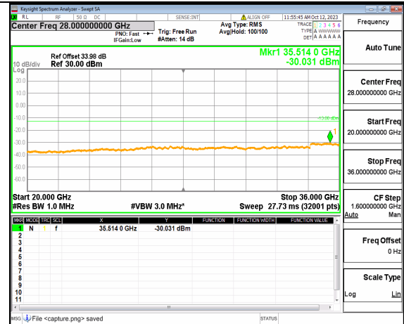
5A_n77(3450-3550MHz) (20GHz-36GHz) 60M DFT-s-OFDM QPSK Outer_Full Mid
