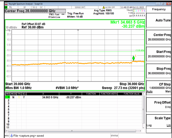
5A_n77(3450-3550MHz) (20GHz-36GHz) 60M DFT-s-OFDM QPSK Outer_Full Low
