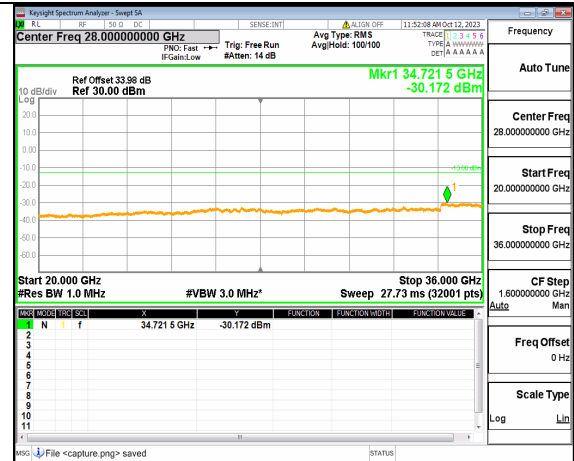
5A_n77(3450-3550MHz) (20GHz-36GHz) 60M DFT-s-OFDM BPSK Outer_Full Mid
