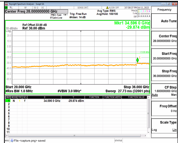
5A_n77(3450-3550MHz) (20GHz-36GHz) 40M DFT-s-OFDM QPSK Edge_1RB_Left Mid
