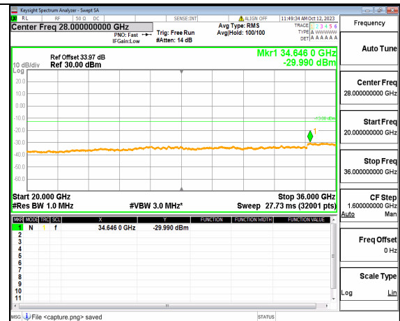
5A_n77(3450-3550MHz) (20GHz-36GHz) 60M DFT-s-OFDM QPSK Edge_1RB_Left Low
