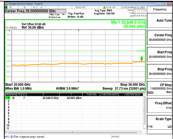
5A_n77(3450-3550MHz) (20GHz-36GHz) 60M DFT-s-OFDM BPSK Edge_1RB_Left Mid
