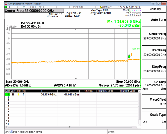
5A_n77(3450-3550MHz) (20GHz-36GHz) 60M DFT-s-OFDM QPSK Edge_1RB_Left Mid
