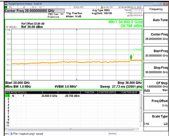
5A_n77(3450-3550MHz) (20GHz-36GHz) 30M DFT-s-OFDM QPSK Edge_1RB_Left High
