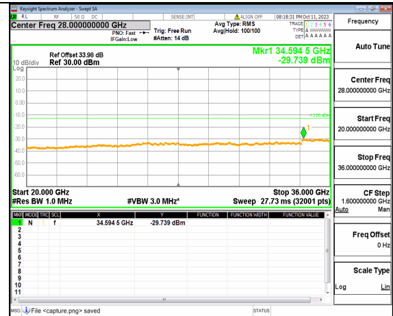
5A_n77(3450-3550MHz) (20GHz-36GHz) 50M DFT-s-OFDM BPSK Edge_1RB_Left Mid
