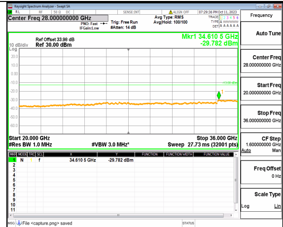
5A_n77(3450-3550MHz) (20GHz-36GHz) 30M DFT-s-OFDM BPSK Outer_Full Mid
