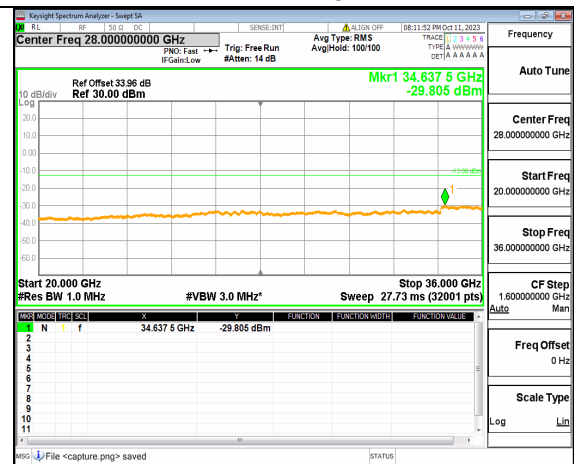
5A_n77(3450-3550MHz) (20GHz-36GHz) 50M DFT-s-OFDM BPSK Edge_1RB_Right Low
