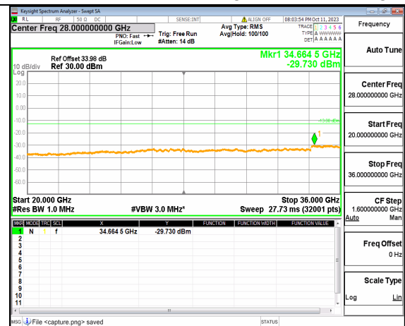
5A_n77(3450-3550MHz) (20GHz-36GHz) 40M DFT-s-OFDM BPSK Edge_1RB_Right High
