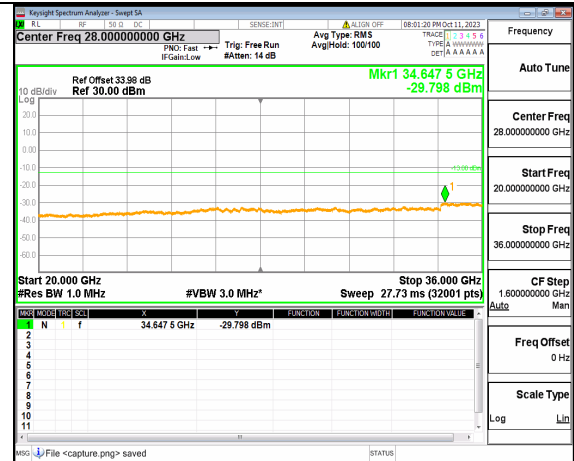
5A_n77(3450-3550MHz) (20GHz-36GHz) 40M DFT-s-OFDM BPSK Outer_Full High
