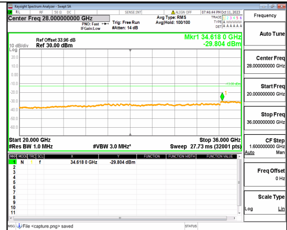
5A_n77(3450-3550MHz) (20GHz-36GHz) 40M DFT-s-OFDM BPSK Edge_1RB_Left Low
