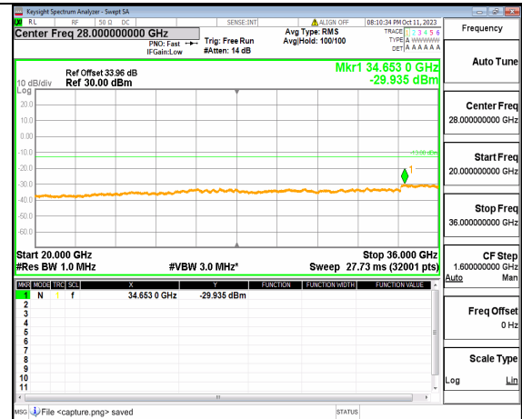
5A_n77(3450-3550MHz) (20GHz-36GHz) 50M DFT-s-OFDM BPSK Edge_1RB_Left Low
