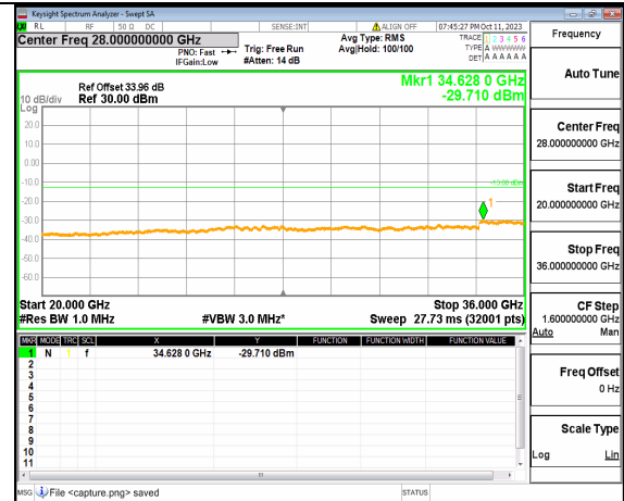
5A_n77(3450-3550MHz) (20GHz-36GHz) 40M DFT-s-OFDM BPSK Outer_Full Low
