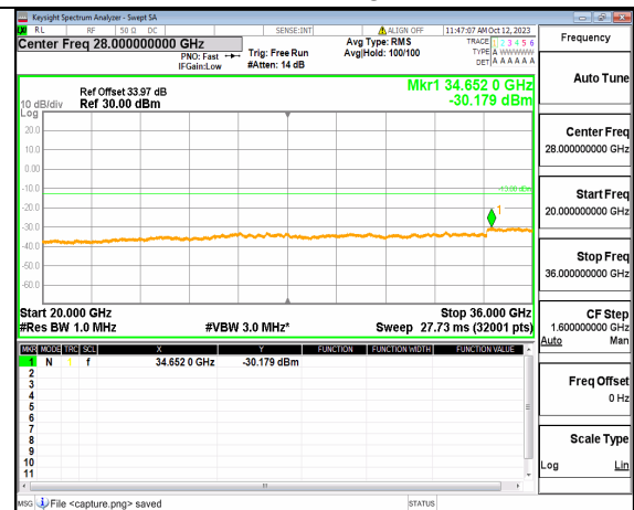
5A_n77(3450-3550MHz) (20GHz-36GHz) 60M DFT-s-OFDM BPSK Edge_1RB_Right Low
