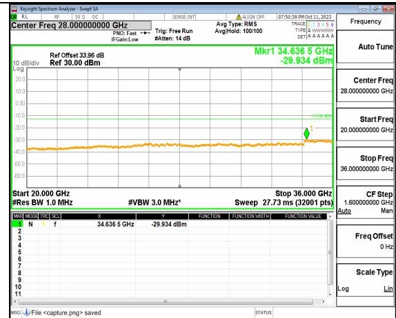
5A_n77(3450-3550MHz) (20GHz-36GHz) 40M DFT-s-OFDM QPSK Edge_1RB_Left Low
