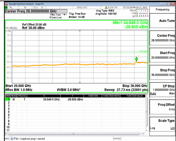
5A_n77(3450-3550MHz) (20GHz-36GHz) 30M DFT-s-OFDM QPSK Outer_Full Mid
