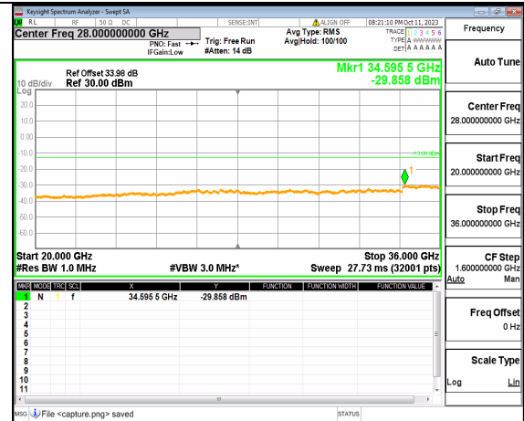
5A_n77(3450-3550MHz) (20GHz-36GHz) 50M DFT-s-OFDM QPSK Outer_Full Mid
