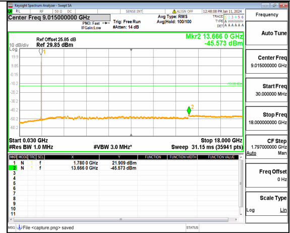
13A_n66 (30MHz-18GHz) 10M DFT-s-OFDM BPSK Inner_1RB_Right High
