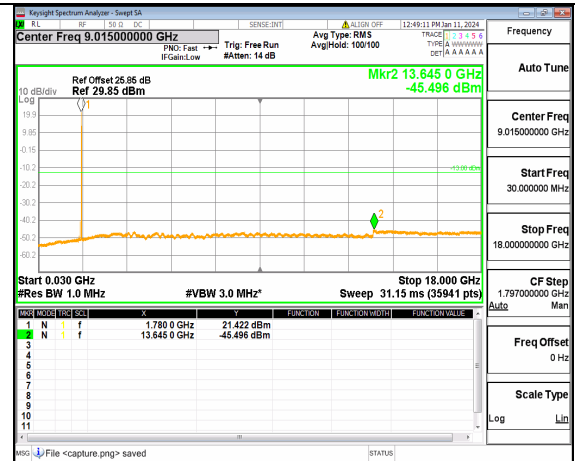
13A_n66 (30MHz-18GHz) 10M DFT-s-OFDM QPSK Inner_1RB_Right High
