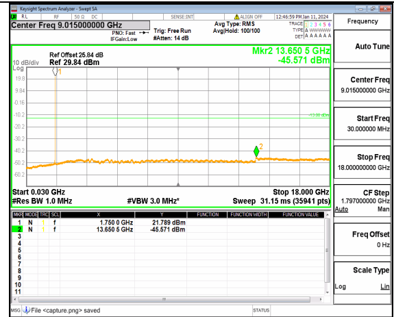
13A_n66 (30MHz-18GHz) 10M DFT-s-OFDM QPSK Inner_1RB_Right Mid
