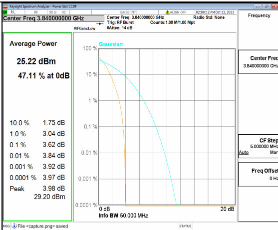
5A_n77(3700-3980MHz) 50M DFT-s-OFDM BPSK Outer_Full Mid
