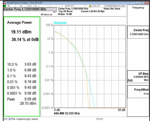
5A_n77(3700-3980MHz) 50M CP-OFDM 256QAM Outer_Full Low
