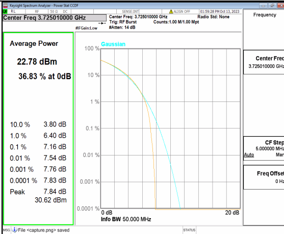
5A_n77(3700-3980MHz) 50M CP-OFDM QPSK Outer_Full Low
