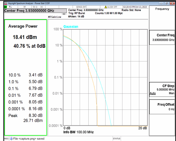
5A_n77(3700-3980MHz) 100M DFT-s-OFDM 256QAM Outer_Full High
