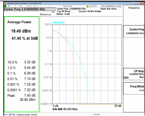
5A_n77(3700-3980MHz) 80M DFT-s-OFDM 256QAM Outer_Full High
