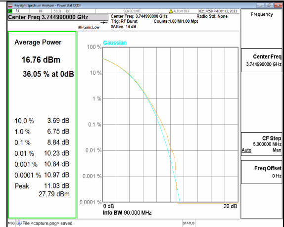
5A_n77(3700-3980MHz) 90M CP-OFDM 256QAM Outer_Full Low
