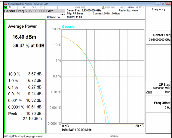
5A_n77(3700-3980MHz) 100M CP-OFDM 256QAM Outer_Full High
