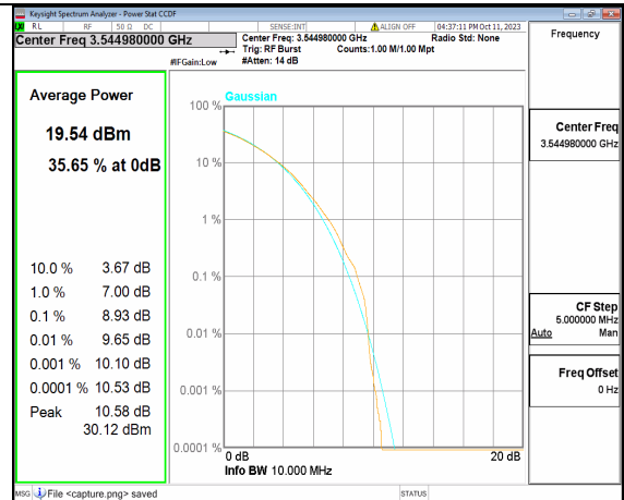
5A_n77(3450-3550MHz) 10M CP-OFDM 256QAM Outer_Full High
