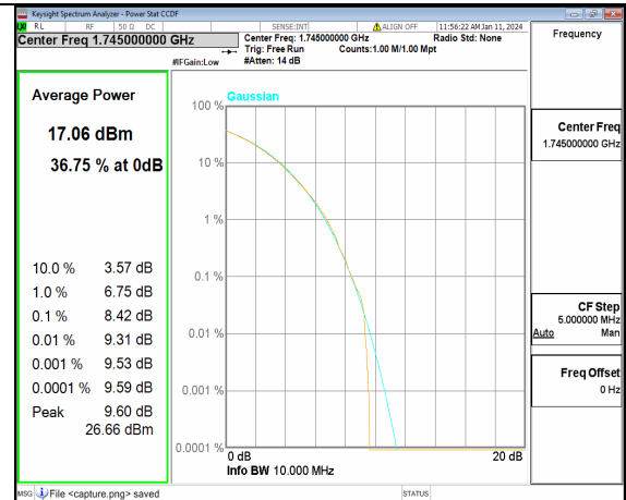
13A_n66 10M CP-OFDM 256QAM Outer_Full Mid
