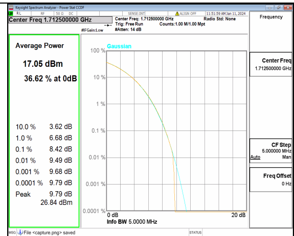
13A_n66 5M CP-OFDM 256QAM Outer_Full Low
