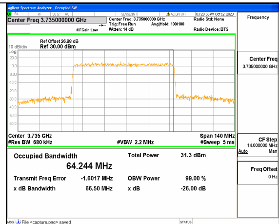
5A_n77(3700-3980MHz) 70M DFT-s-OFDM QPSK Outer_Full Low
