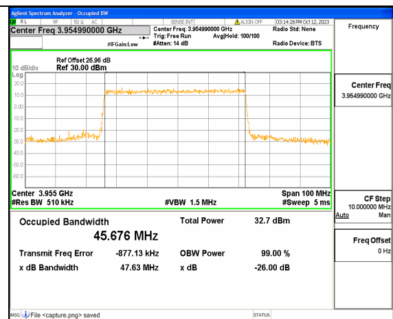
5A_n77(3700-3980MHz) 50M DFT-s-OFDM 64QAM Outer_Full High
