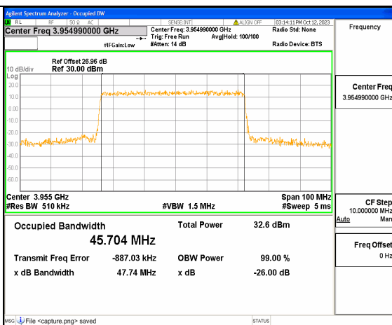
5A_n77(3700-3980MHz) 50M DFT-s-OFDM 16QAM Outer_Full High
