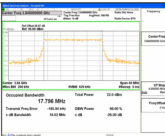
5A_n77(3700-3980MHz) 20M DFT-s-OFDM 16QAM Outer_Full Mid
