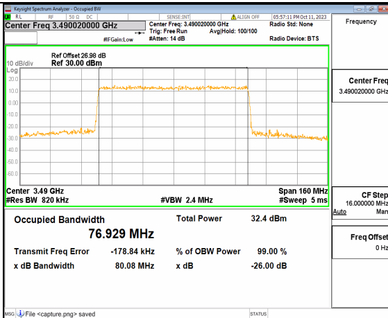
5A_n77(3450-3550MHz) 80M DFT-s-OFDM 16QAM Outer_Full Low
