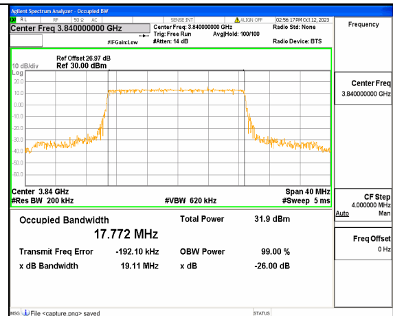
5A_n77(3700-3980MHz) 20M DFT-s-OFDM QPSK Outer_Full Mid
