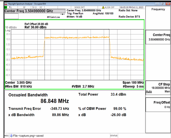
5A_n77(3450-3550MHz) 90M DFT-s-OFDM QPSK Outer_Full High
