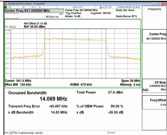
2A_n5 15M CP-OFDM QPSK Outer_Full High
