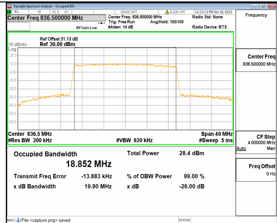
2A_n5 20M CP-OFDM QPSK Outer_Full Mid
