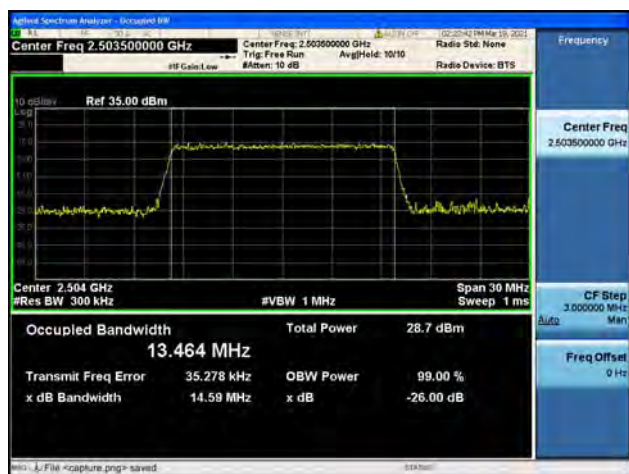
Band41 / 15MHz / Mid CH / 16QAM
