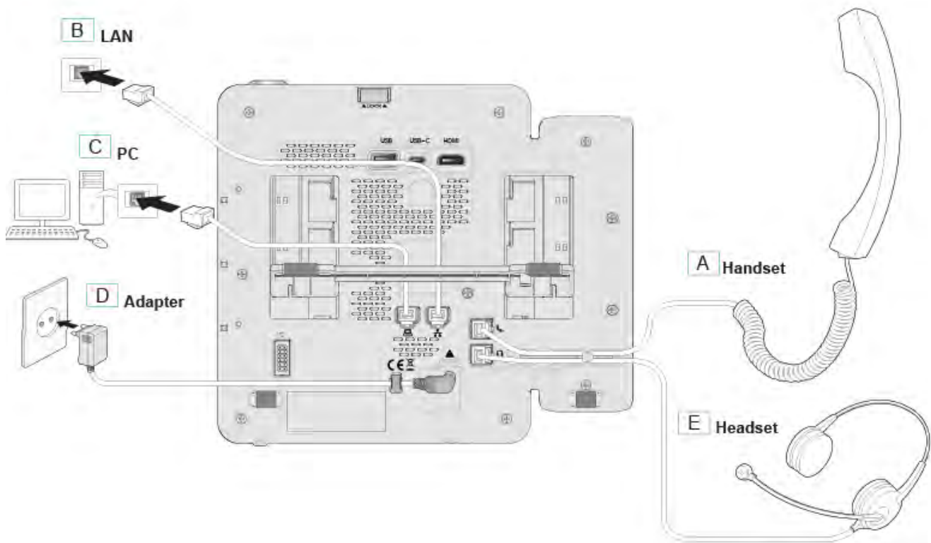
Figure 2-3 1080i Installation
