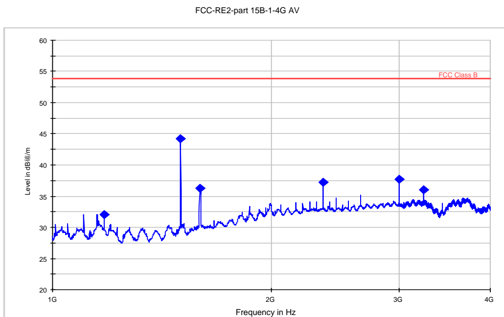
Figure A.2 Radiated Emission from 1GHz to 4GHz (Set.1, USB mode)
