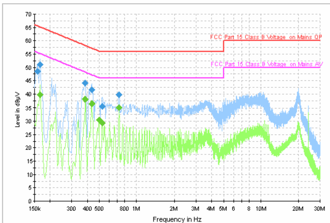
Figure A.6 Conducted Emission (Set.1, USB mode)
