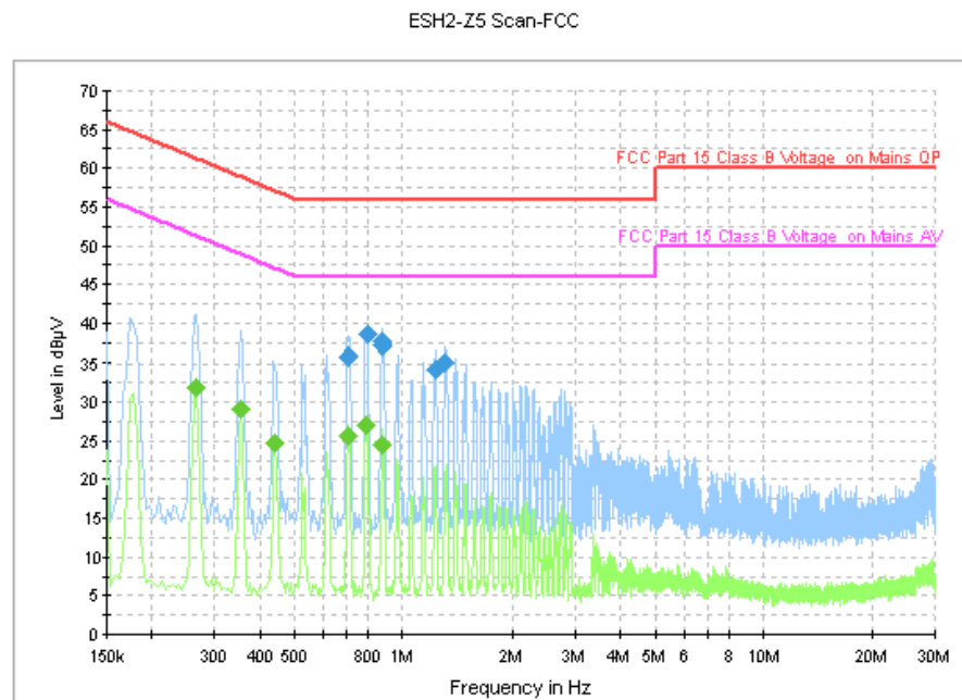
Fig. 94 AC Power line Conducted Emission (Idle, AE1)
