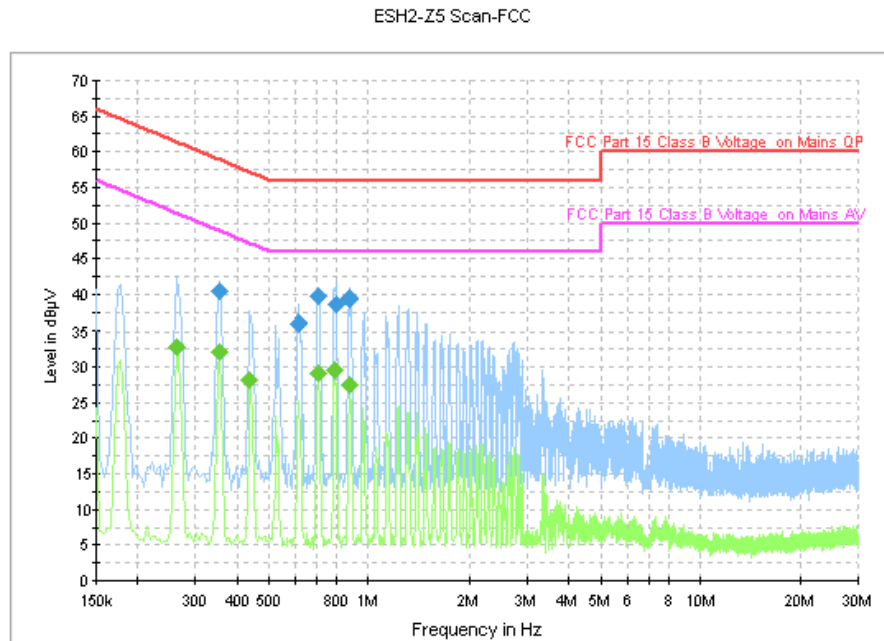
Fig. 93 AC Power line Conducted Emission (Traffic, AE1)
