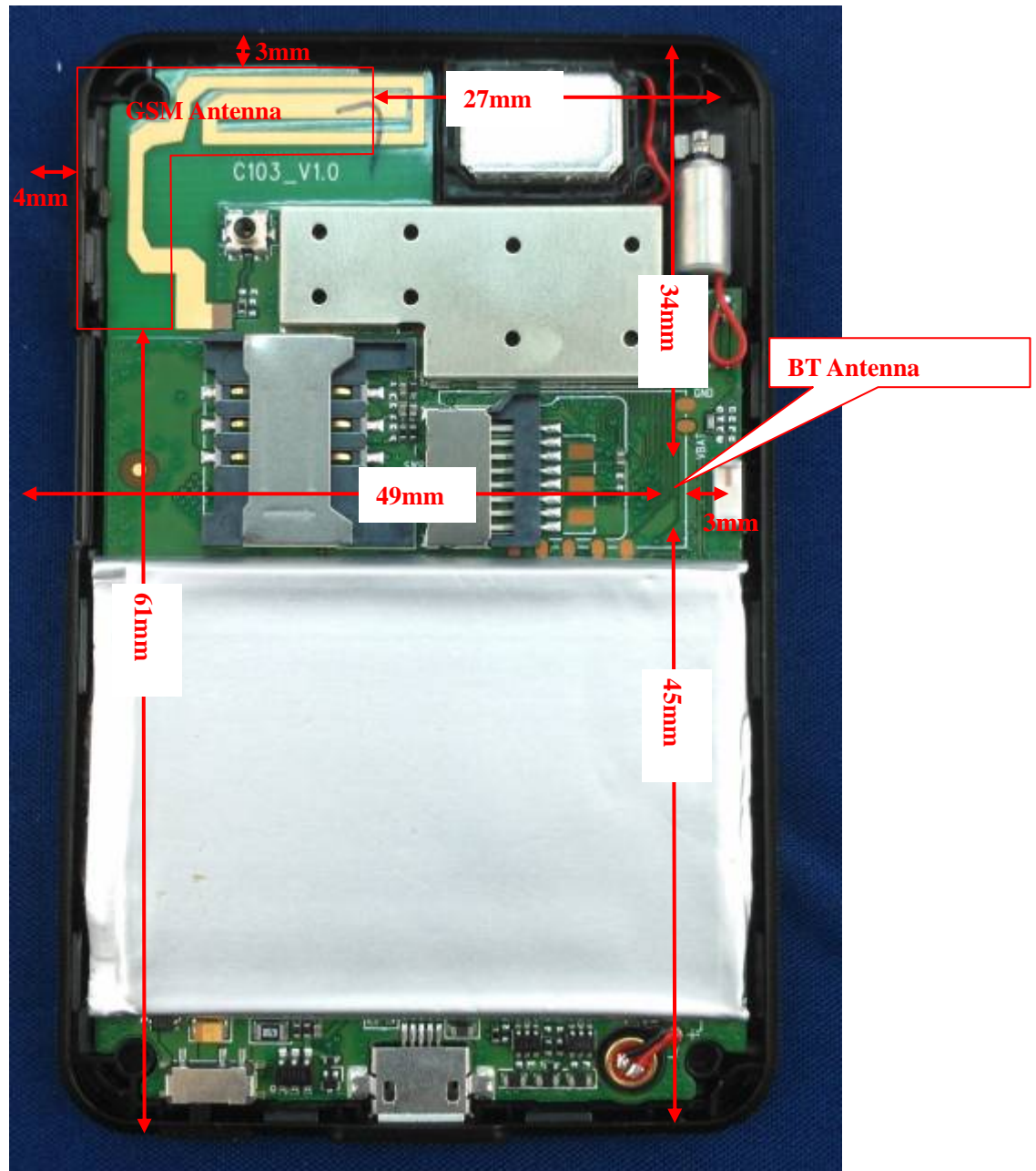
Picture 11.1 Antenna Locations
