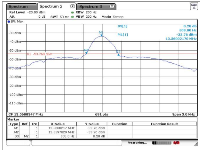
20 dB Bandwidth
