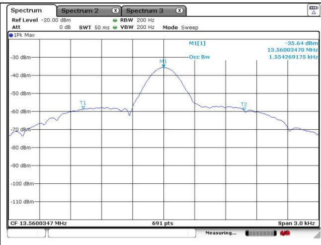
99 % Bandwidth
