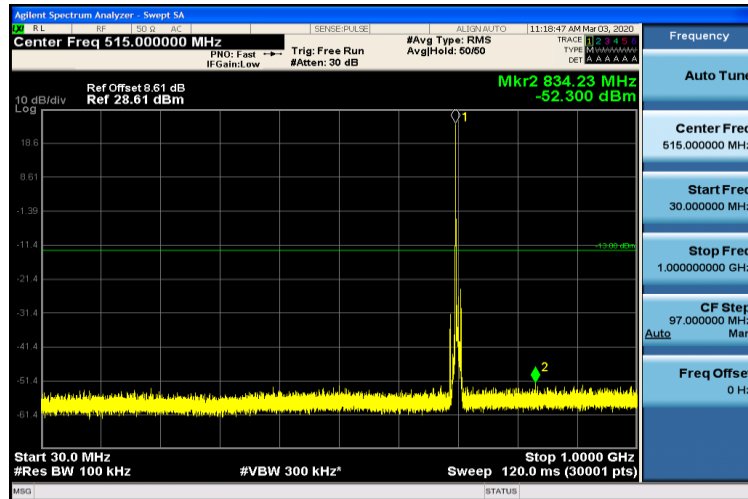
Band17-5MHz-16QAM-23755-1RB#0-30~1000MHz
