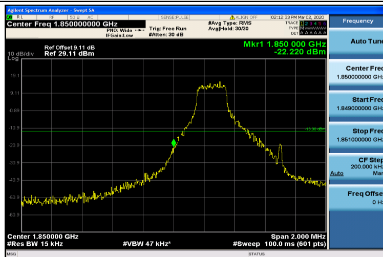
Band2-1.4MHz-16QAM-18607-1RB#0
