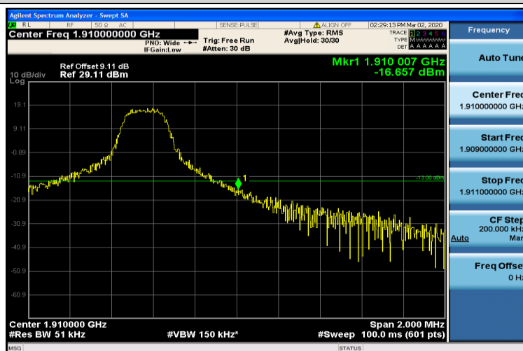
Band2-5MHz-16QAM-19175-1RB#24
