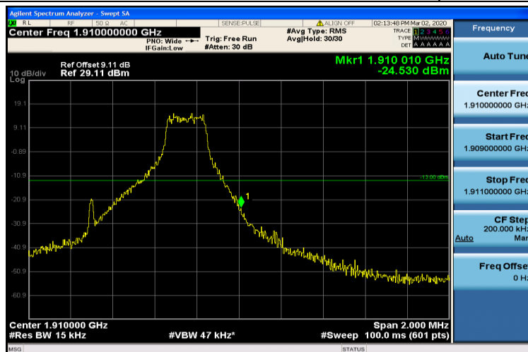
Band2-1.4MHz-16QAM-19193-1RB#5
