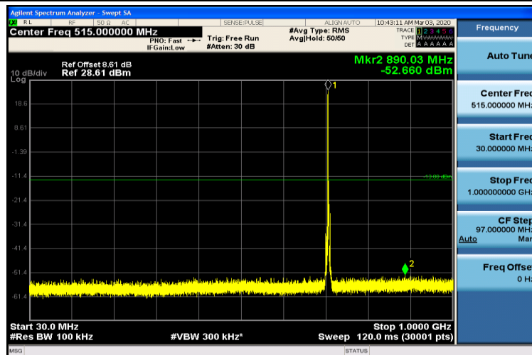
Band12-3MHz-16QAM-23165-1RB#0-30~1000MHz
