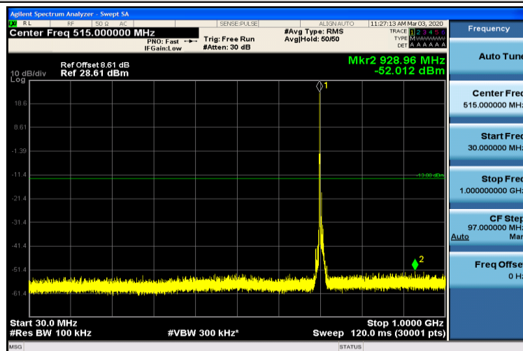
Band17-10MHz-QPSK-23800-1RB#0-30~1000MHz
