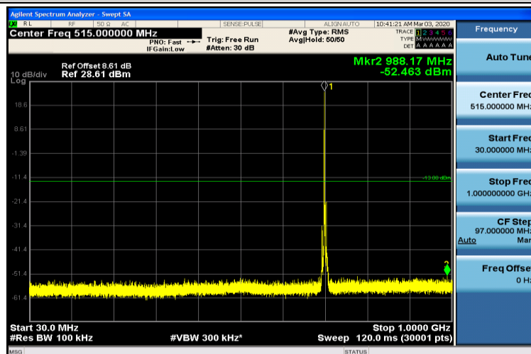
Band12-3MHz-QPSK-23095-1RB#0-30~1000MHz
