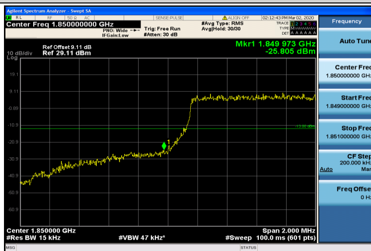
Band2-1.4MHz-QPSK-18607-6RB#0
