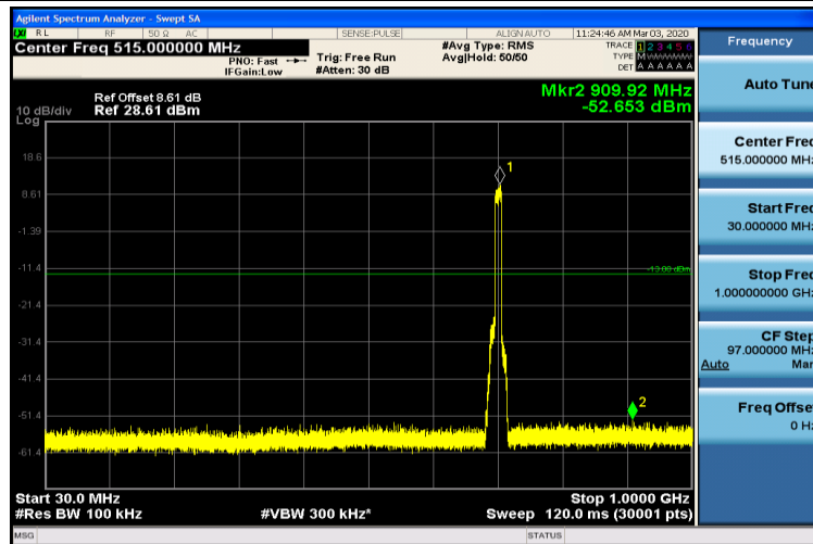
Band17-10MHz-QPSK-23780-1RB#0-30~1000MHz
