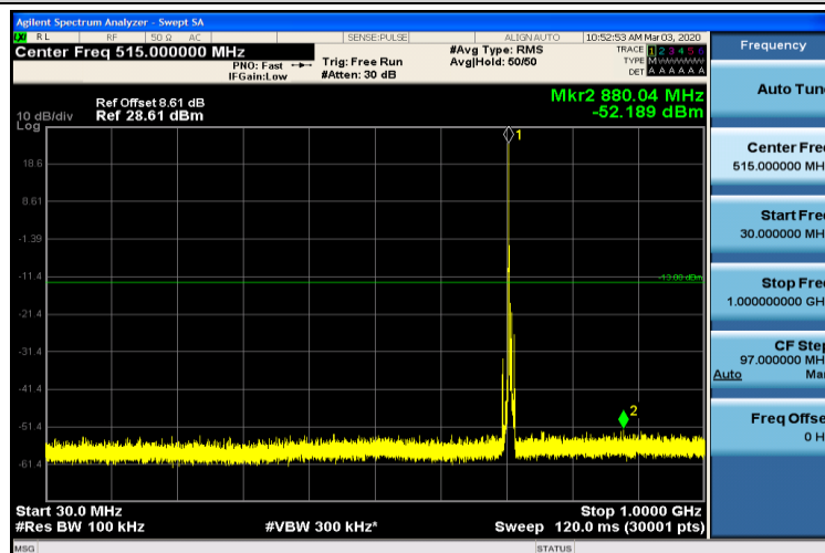
Band12-5MHz-16QAM-23155-1RB#0-30~1000MHz
