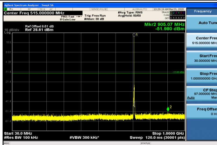
Band12-1.4MHz-QPSK-23173-1RB#0-30~1000MHz
