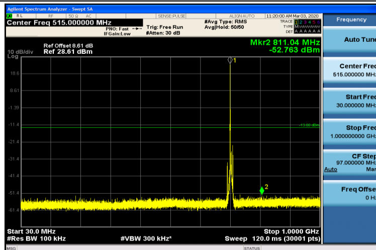
Band17-5MHz-16QAM-23790-1RB#0-30~1000MHz
