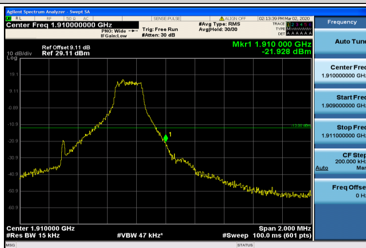
Band2-1.4MHz-QPSK-19193-1RB#5
