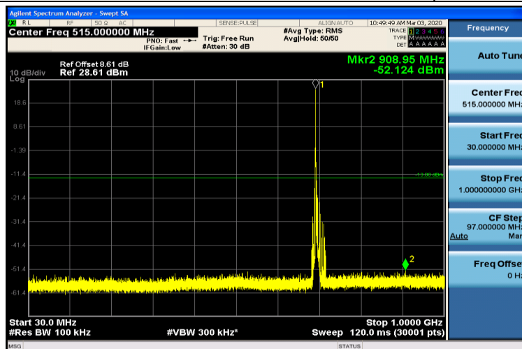
Band12-5MHz-QPSK-23035-1RB#0-30~1000MHz
