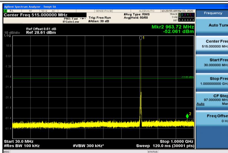
Band12-1.4MHz-16QAM-23173-1RB#0-30~1000MHz
