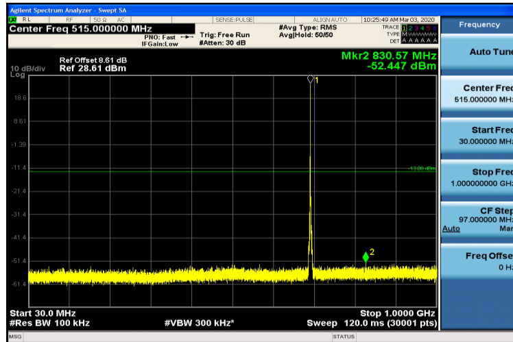
Band12-1.4MHz-16QAM-23017-1RB#0-30~1000MHz
