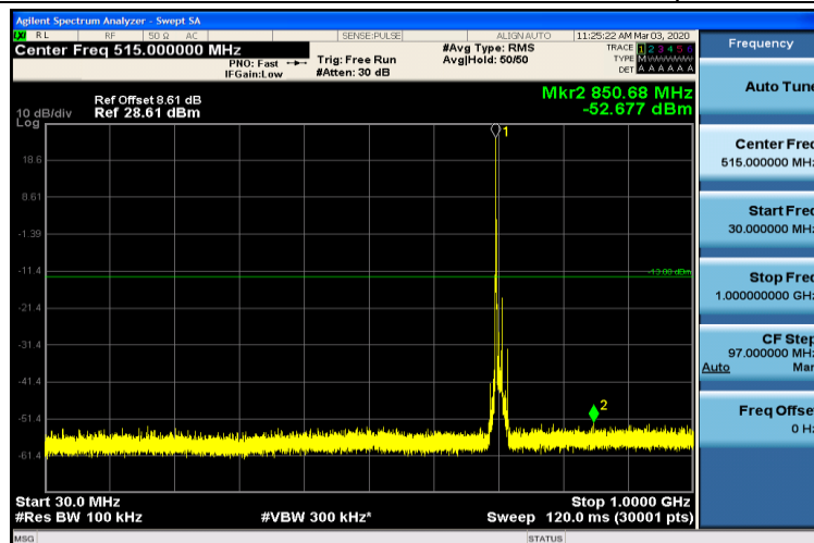
Band17-10MHz-16QAM-23780-1RB#0-30~1000MHz
