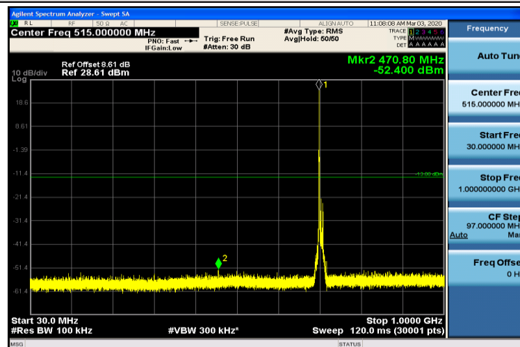
Band12-10MHz-QPSK-23130-1RB#0-30~1000MHz
