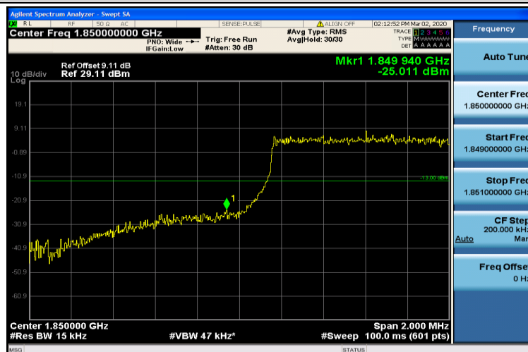
Band2-1.4MHz-16QAM-18607-6RB#0
