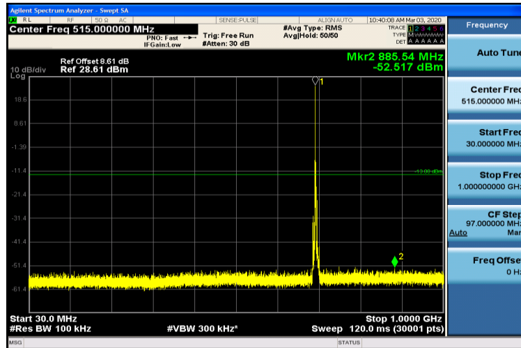
Band12-3MHz-QPSK-23025-1RB#0-30~1000MHz
