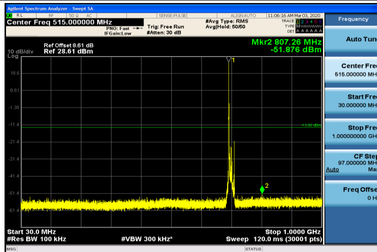
Band12-10MHz-16QAM-23060-1RB#0-30~1000MHz
