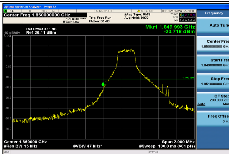
Band2-1.4MHz-QPSK-18607-1RB#0
