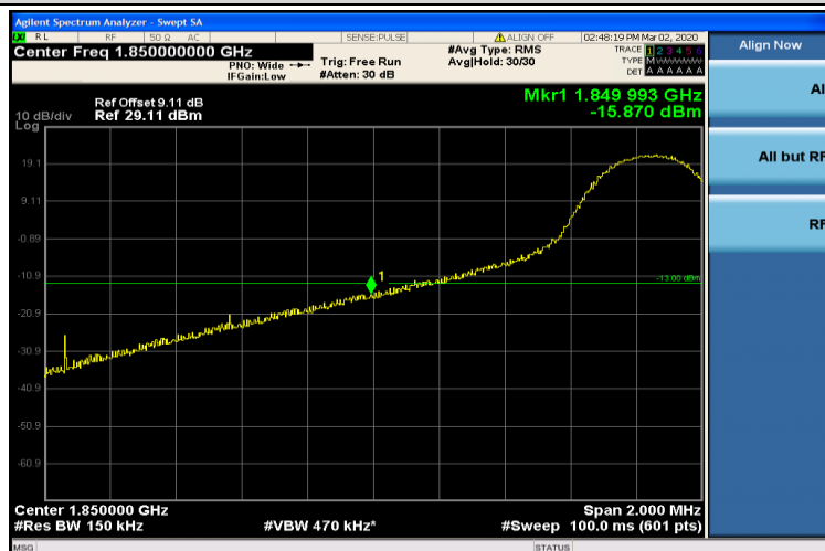
Band2-15MHz-QPSK-18675-1RB#0
