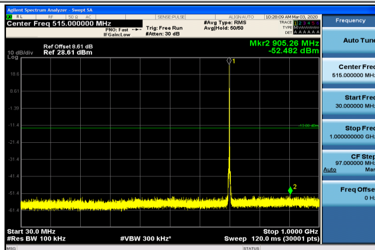
Band12-1.4MHz-16QAM-23095-1RB#0-30~1000MHz
