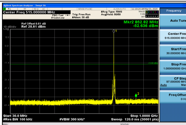
Band17-5MHz-QPSK-23790-1RB#0-30~1000MHz
