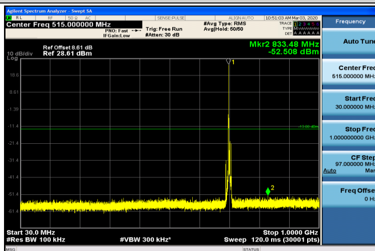
Band12-5MHz-QPSK-23095-1RB#0-30~1000MHz
