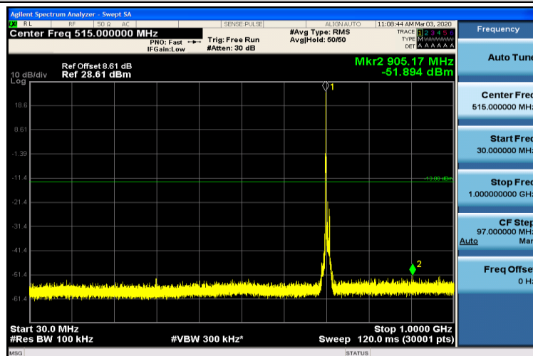
Band12-10MHz-16QAM-23130-1RB#0-30~1000MHz
