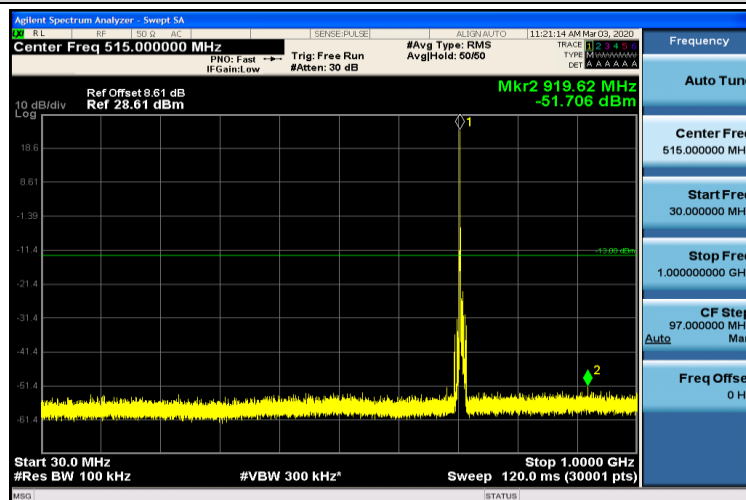
Band17-5MHz-16QAM-23825-1RB#0-30~1000MHz
