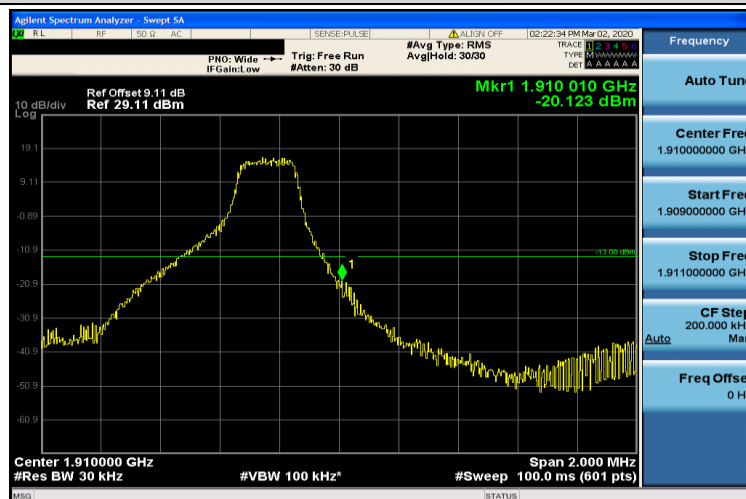
Band2-3MHz-16QAM-19185-1RB#14
