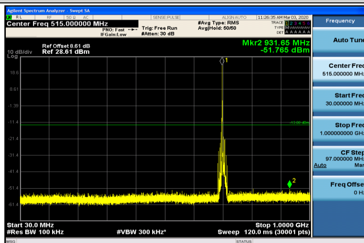
Band17-10MHz-16QAM-23790-1RB#0-30~1000MHz
