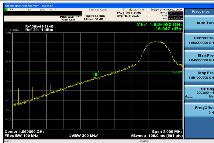
Band2-10MHz-16QAM-18650-1RB#0
