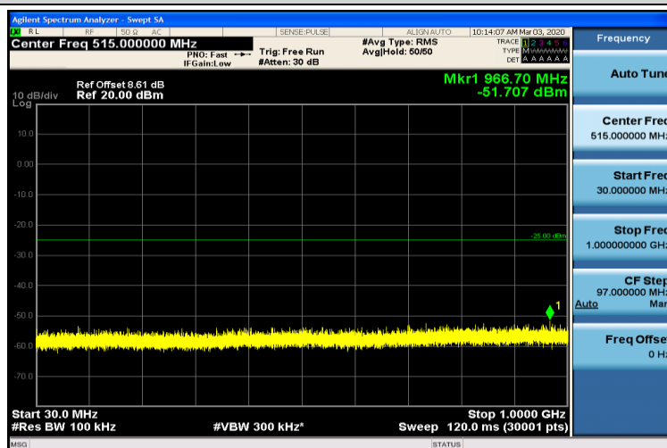
Band7-20MHz-16QAM-21350-1RB#0-30~1000MHz
