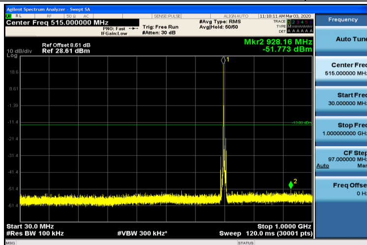
Band17-5MHz-QPSK-23755-1RB#0-30~1000MHz
