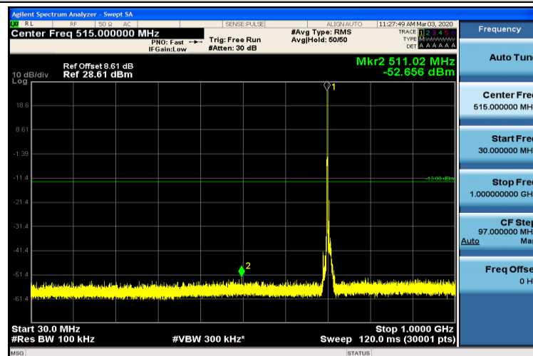
Band17-10MHz-16QAM-23800-1RB#0-30~1000MHz
