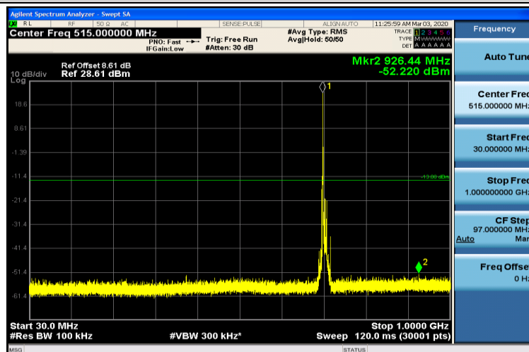
Band17-10MHz-QPSK-23790-1RB#0-30~1000MHz
