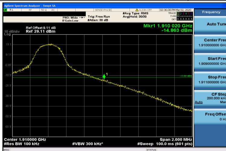
Band2-10MHz-16QAM-19150-1RB#49
