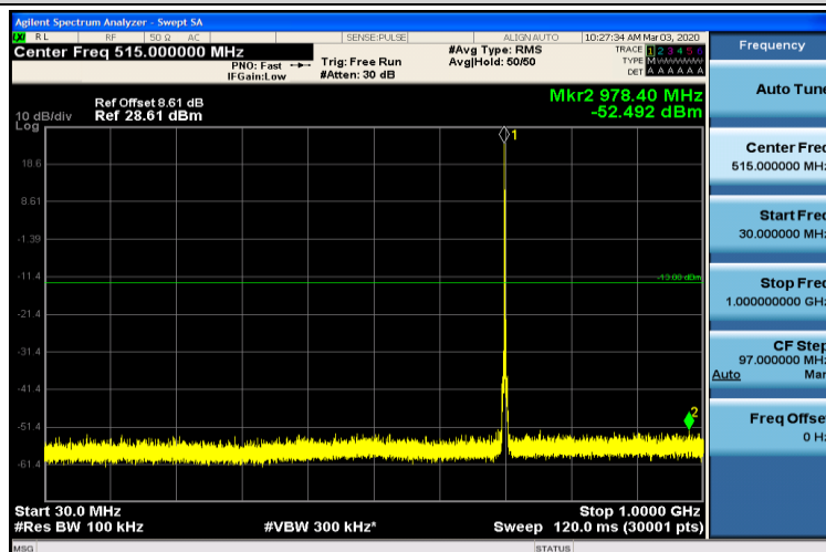
Band12-1.4MHz-QPSK-23095-1RB#0-30~1000MHz
