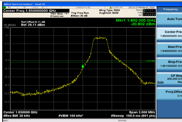
Band2-3MHz-16QAM-18615-1RB#0
