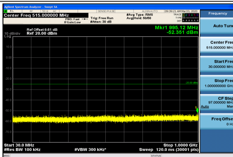
Band7-5MHz-QPSK-21425-1RB#0-30~1000MHz
