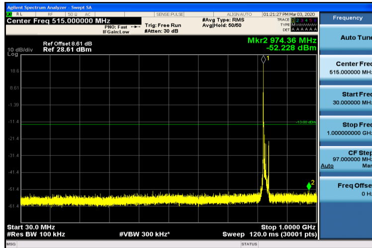
Band5-10MHz-QPSK-20450-1RB#0-30~1000MHz
