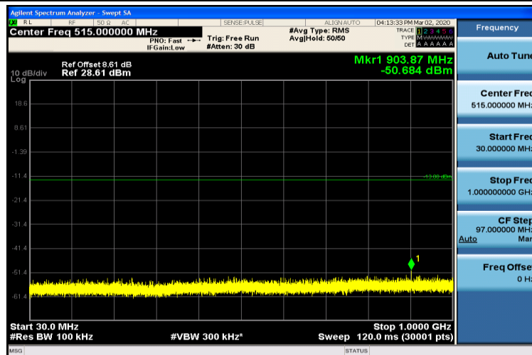
Band4-15MHz-16QAM-20325-1RB#0-30~1000MHz
