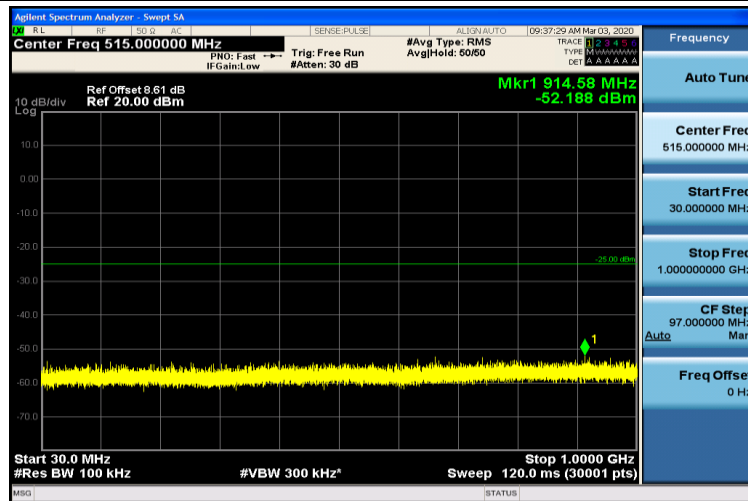
Band7-5MHz-16QAM-20775-1RB#0-30~1000MHz
