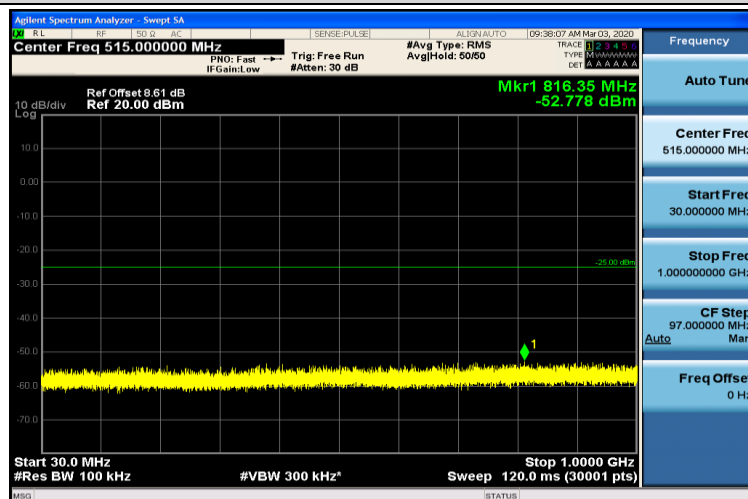
Band7-5MHz-QPSK-21100-1RB#0-30~1000MHz
