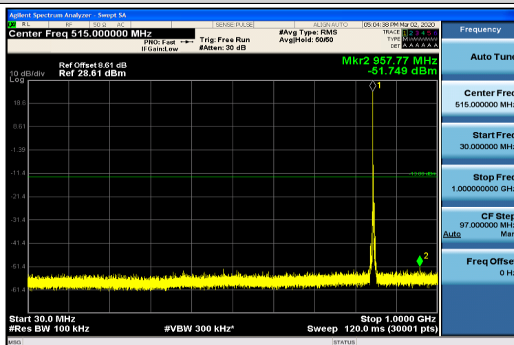
Band5-3MHz-16QAM-20635-1RB#0-30~1000MHz
