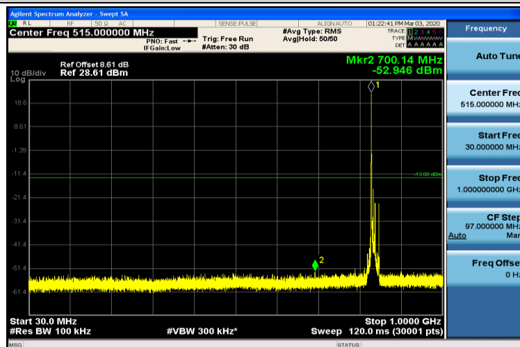
Band5-10MHz-QPSK-20525-1RB#0-30~1000MHz
