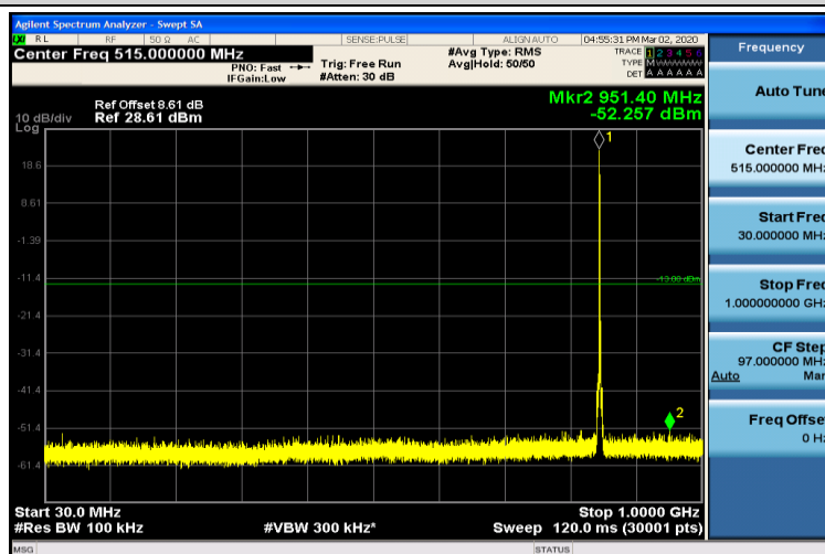
Band5-1.4MHz-QPSK-20643-1RB#0-30~1000MHz
