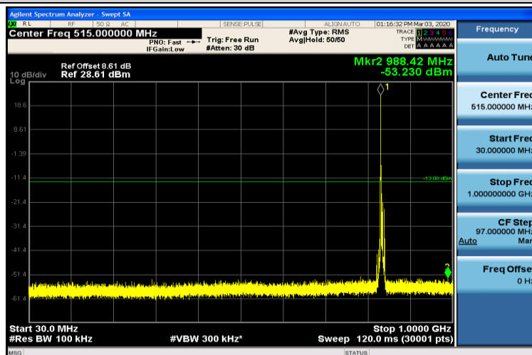
Band5-5MHz-QPSK-20525-1RB#0-30~1000MHz
