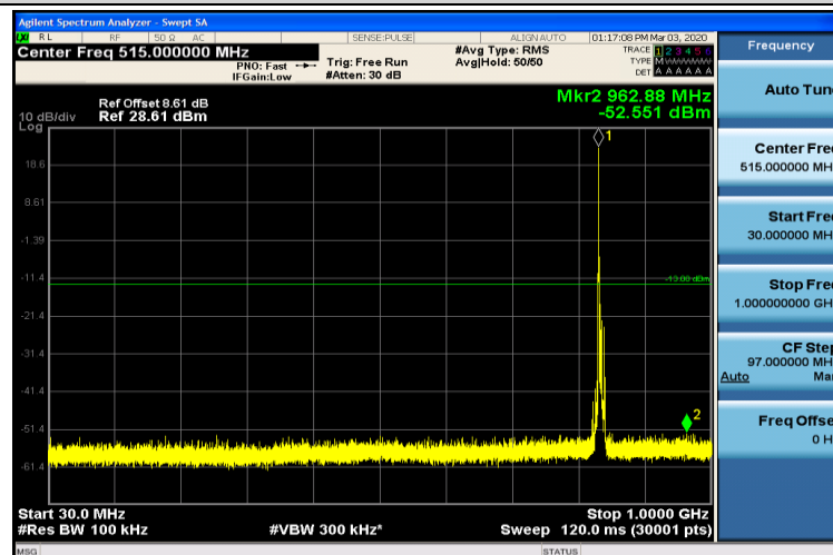
Band5-5MHz-16QAM-20525-1RB#0-30~1000MHz
