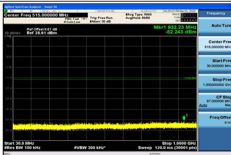
Band4-20MHz-16QAM-20300-1RB#0-30~1000MHz
