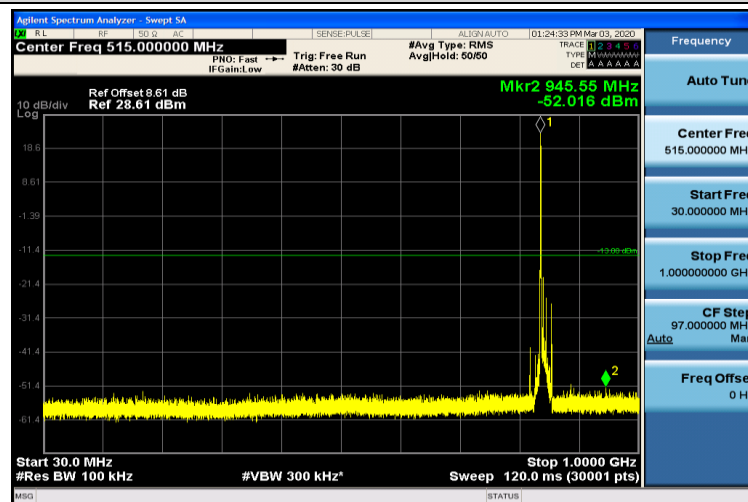
Band5-10MHz-16QAM-20600-1RB#0-30~1000MHz
