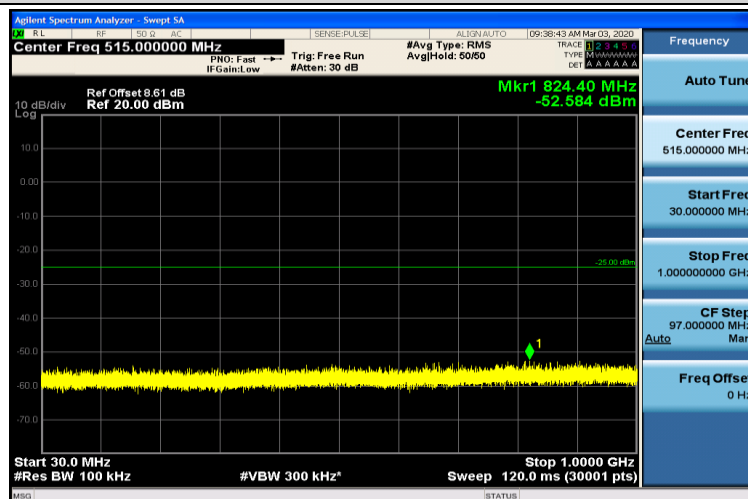
Band7-5MHz-16QAM-21100-1RB#0-30~1000MHz
