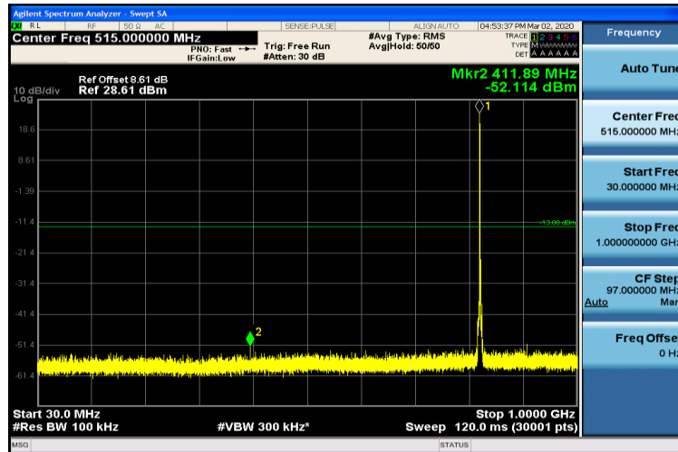
Band5-1.4MHz-16QAM-20407-1RB#0-30~1000MHz
