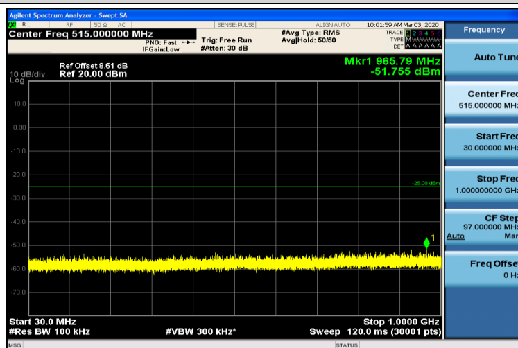
Band7-15MHz-16QAM-21375-1RB#0-30~1000MHz
