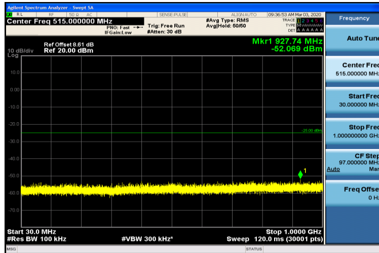
Band7-5MHz-QPSK-20775-1RB#0-30~1000MHz
