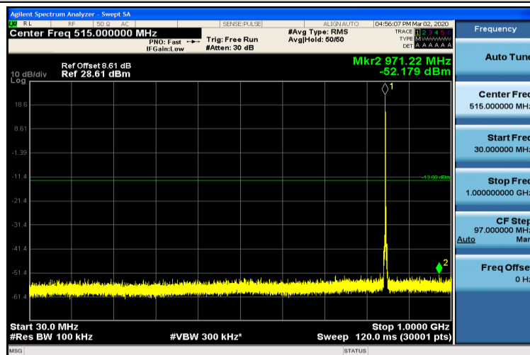
Band5-1.4MHz-16QAM-20643-1RB#0-30~1000MHz
