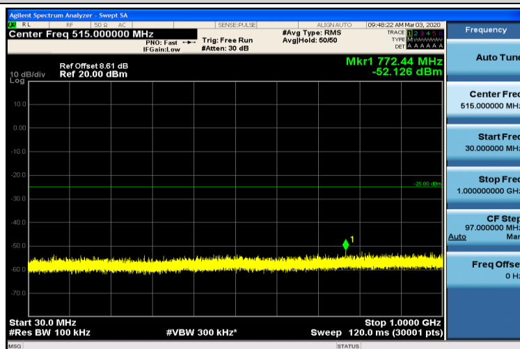
Band7-10MHz-16QAM-21400-1RB#0-30~1000MHz
