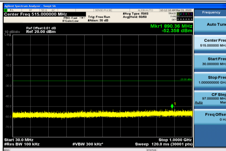
Band7-20MHz-QPSK-21100-1RB#0-30~1000MHz
