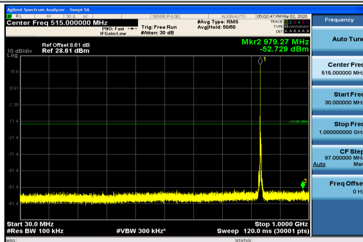
Band5-3MHz-QPSK-20525-1RB#0-30~1000MHz
