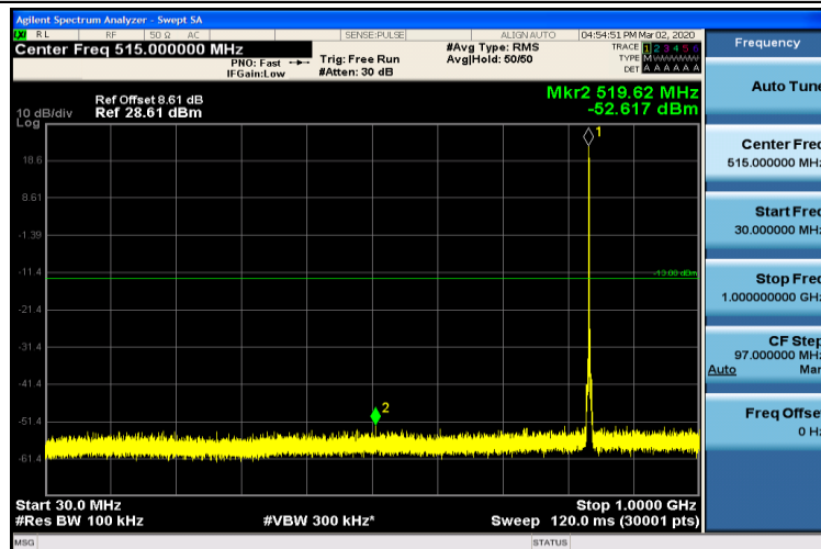
Band5-1.4MHz-16QAM-20525-1RB#0-30~1000MHz
