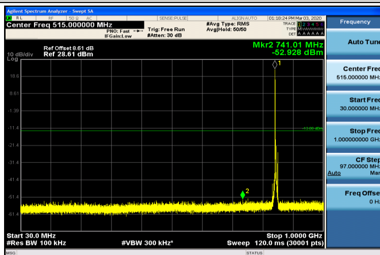
Band5-5MHz-16QAM-20625-1RB#0-30~1000MHz
