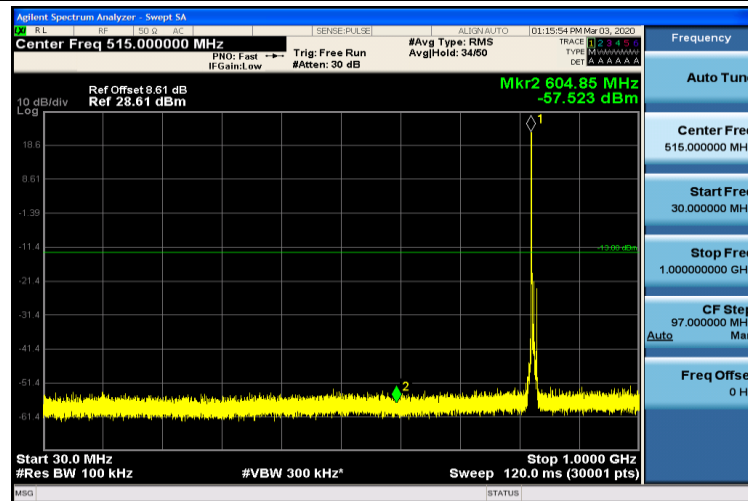
Band5-5MHz-16QAM-20425-1RB#0-30~1000MHz
