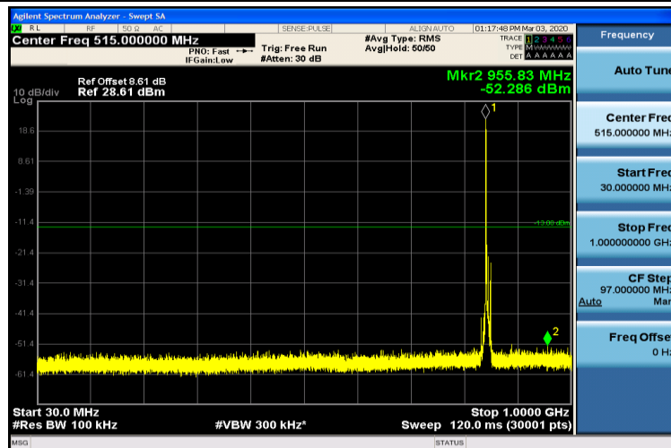
Band5-5MHz-QPSK-20625-1RB#0-30~1000MHz
