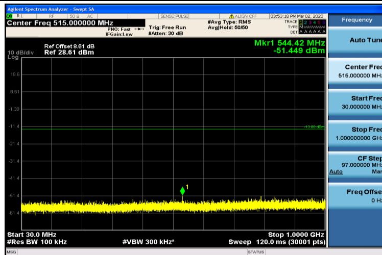
Band4-1.4MHz-16QAM-20393-1RB#0-30~1000MHz
