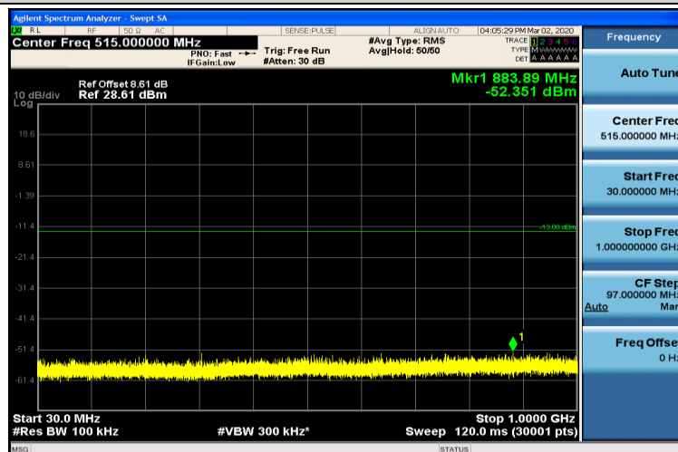
Band4-10MHz-QPSK-20175-1RB#0-30~1000MHz
